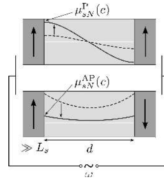
FIG. 1: Scheme of an FNF spin valve. The spacer N region has width d and the sizes of the ferromagnetic electrodes are assumed greater than the corresponding spin diffusion length L_s . In the dc regime the parallel configurations results in smaller spin accumulation (dashed line) than in the antiparallel one, demonstrated by the positive dc spin-valve magnetoresistance. In the ac regime, this can be reversed (solid): at certain frequency ranges there can be a resonant spin amplification in the parallel and spin depletion in the antiparallel configuration, resulting in a negative ac magnetoresistance.
