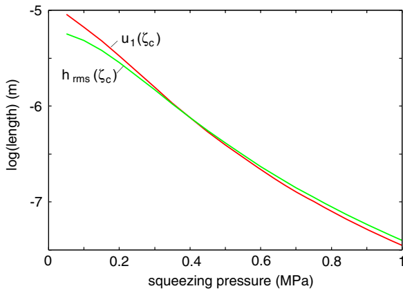
Figure 12. The interfacial separation u_c = u_1(\zeta_c) and the rms roughness h_{\text{rms}}(\zeta_c) in the critical constriction of the percolation channel, as a function of the applied normal (or squeezing) pressure P_0 . Results are shown for self-affine fractal surfaces with the Hurst exponent H = 0.8 (or fractal dimension D_f = 2.2 ), and with the root-mean-square roughness (rms) 6 \mu\text{m} .
