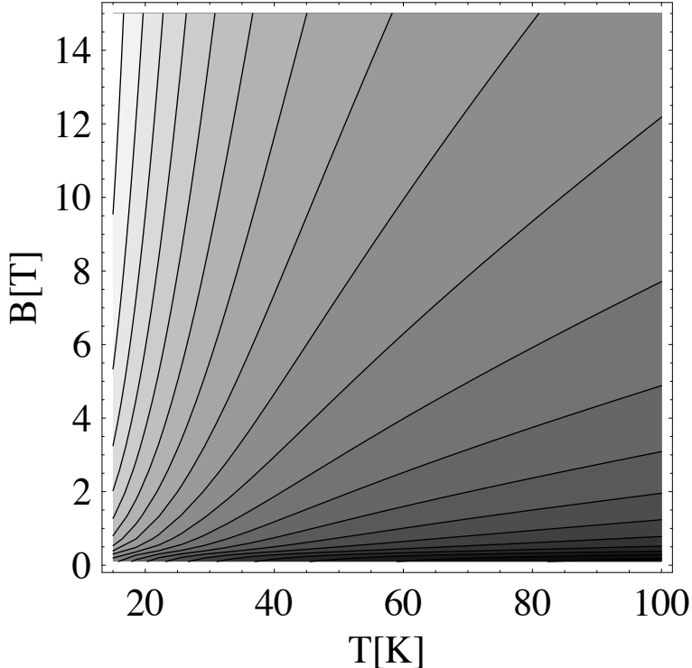
FIG. 3: Contour plot (with logarithmic spacing) of the thermoelectric conductivity \alpha_{xy} (Eq. 2.3) as a function of temperature T and magnetic field B , for parameters \hbar v = 47 \text{ meV \AA} , \delta - \delta_I = 0.025 and \tau_{\text{imp}} = 10^{-12} \text{ s} estimated for LSCO. In the ordered low temperature regime T < T_c \approx 30 \text{ K} , Eq. (2.3) will receive modifications.
