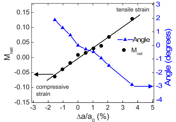
FIG. 5. (Color online) The net magnetic moment per unit cell and the rotation angle of Mn2 sites as functions of the biaxial strain [\Delta a/a_0(\%)] in \text{Mn}_3\text{GaN} , noncollinear \Gamma^{5g} structure.
