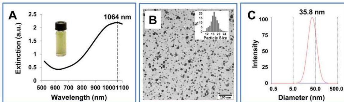
Fig. 1. Characterization of CuS NPs. A) Extinction spectra of 100 µg/mL CuS NPs aqueous solution. Inset: photograph of an aqueous solution of PEG-CuS NPs after storage at 4°C for 6 months in the presence of argon. B) Transmission electron microscopy photograph of CuS NPs. Inset: particle size distribution. C) Hydrodynamic diameter distribution of PEG-CuS NP samples determined by dynamic light scattering measurement immediately after synthesis.
