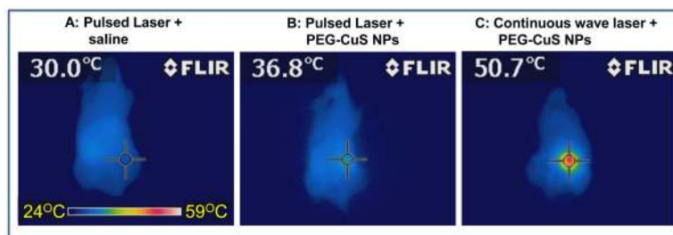
Fig. 6. Representative in vivo infrared thermographic images of 4T1 tumor-bearing mice obtained with or without PEG-CuS NPs followed by irradiation at 1064-nm (at 4.32 W/cm 2 ) with pulsed laser or at 808 nm (at 3 W/cm 2 ) with continuous wave laser light for 2 min.
