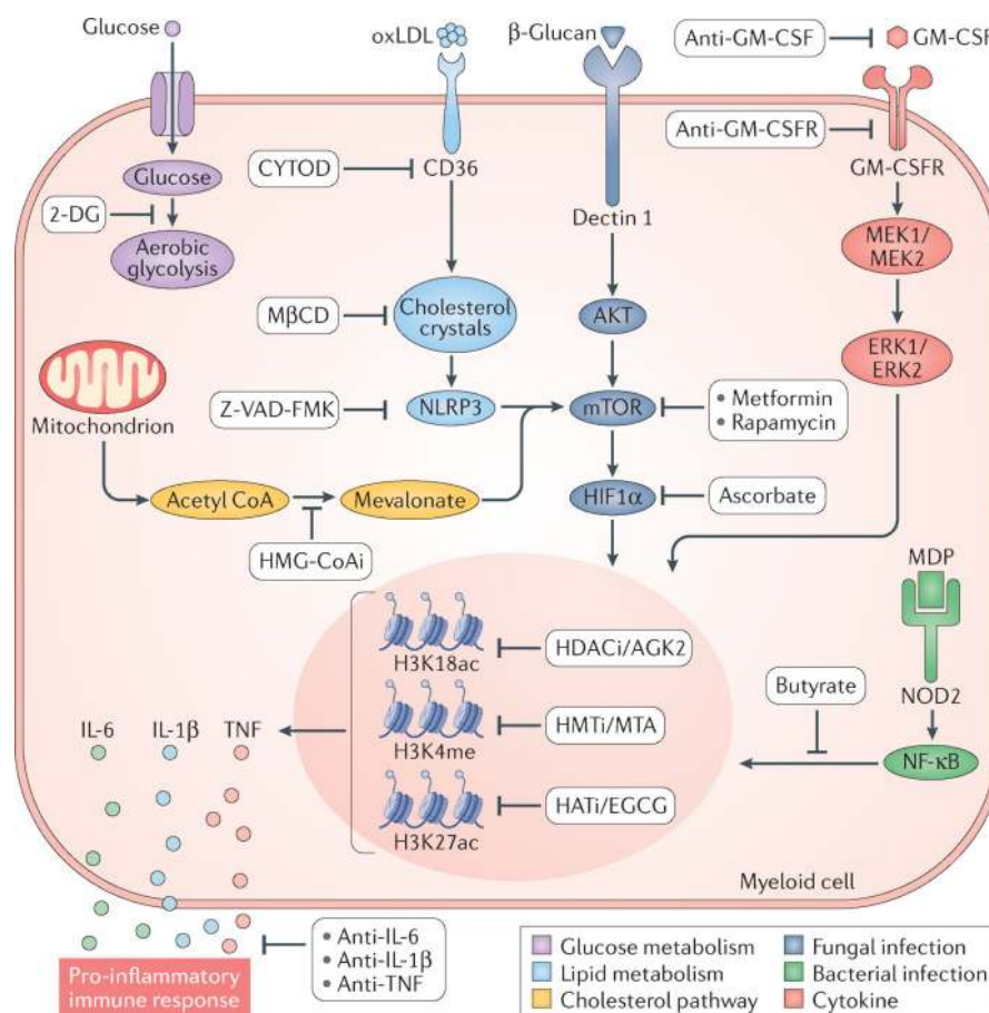
Fig. 3 |. Trained-immunity-regulating pathways.
