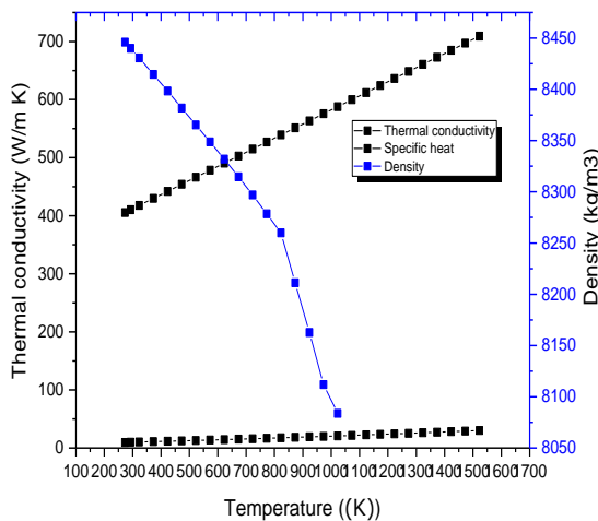
Fig.2: Thermal properties for inconel 625
