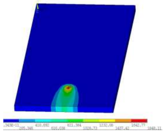
Fig.8: Temperature at Time=10sec
