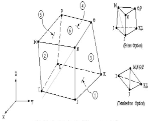
Fig.3: Solid70 3-D Thermal Solid
