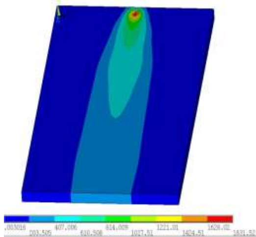
Fig.13: Temperature at Time=50sec
