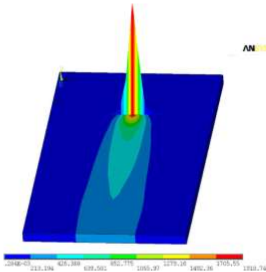
Fig.12: Nodel Temperature of Weldment
