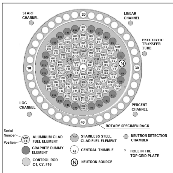
FIG. 2: Current horizontal cross-section of TRIGA IPR-R1 reactor core [3].
