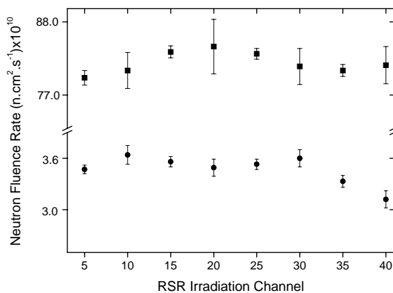
FIG. 4: Thermal (square) and epithermal (circle) neutron fluence rates at eight irradiation channels of the TRIGA IPR-R1 Rotary Specimen Rack.
