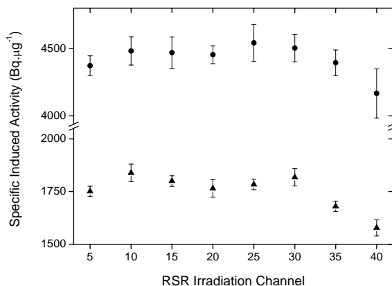
FIG. 3: Specific induced activity on bare (circles) and cadmium-covered (triangles) probes irradiated in the TRIGA IPR-R1 Rotary Specimen Rack.
