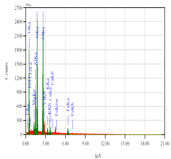
(c). (LiCl) 0.5 (MMT) 0.5 sample
