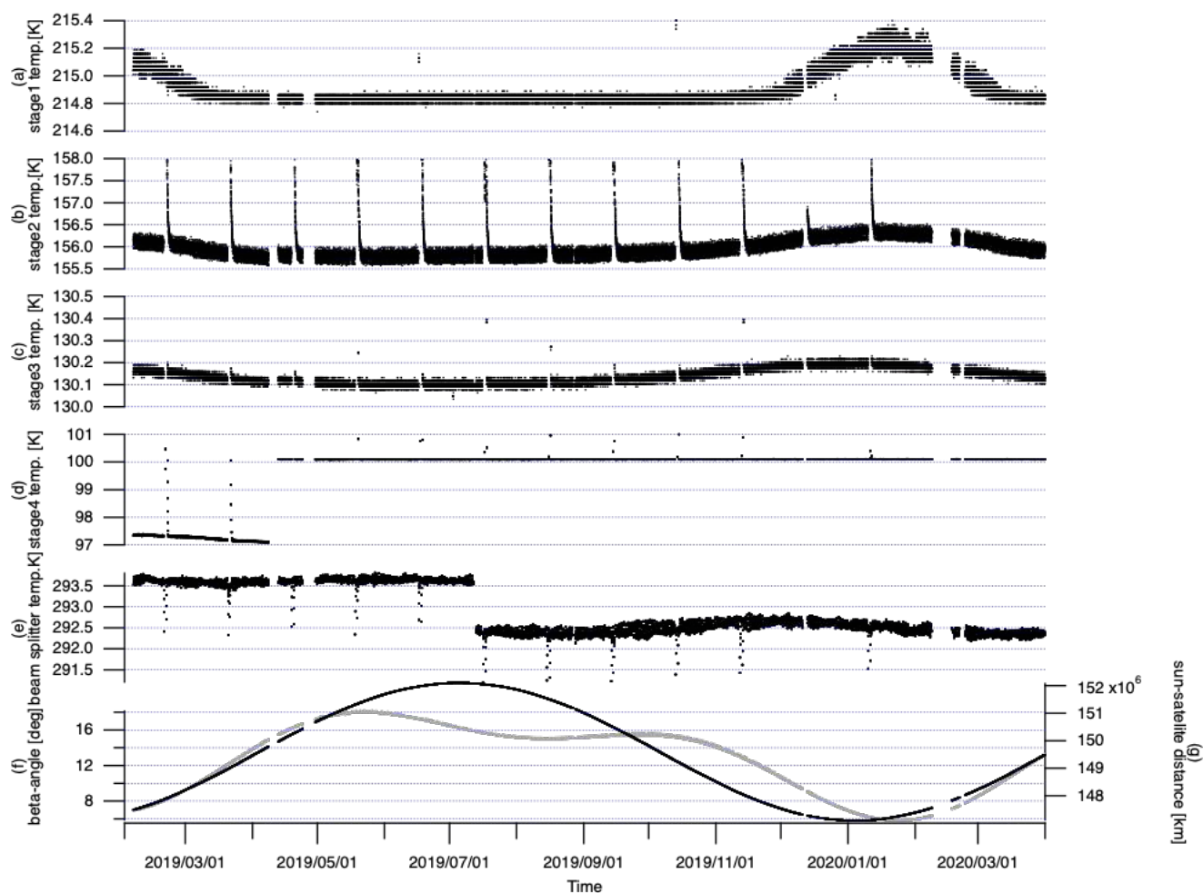
855 Figure 9. Time series of temperatures (a)cooler stage1, (b)cooler stage2, (c)cooler stage3, (d)cooler stage4, (e)beam splitter on interferometer, (f) satellite beta-angle (grey with left axis) and (g)sun-satellite distance (black with right axis).
