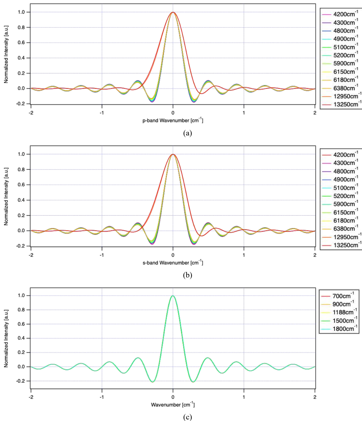
Figure 6. The simulated instrument line shape function (ILS): (a) p-polarization bands for SWIR; (b) s-polarization bands for SWIR; (c) TIR bands.
