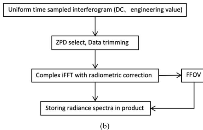
Figure 7. Processing flow for SWIR bands (a) and for TIR bands (b).
