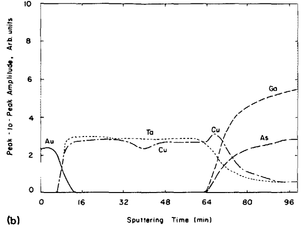
FIG. 8. (a) Schematic AES depth profiles showing the effect of no anneal on Cu 20 at. % Ta barriers on GaAs substrates with Au overlayers. (b) Schematic AES depth profiles showing the effect of anneal to 500 °C on Cu 20 at. % Ta barriers on GaAs substrates with Au overlayer.
