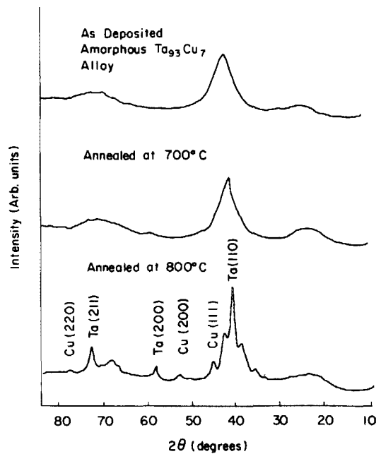
FIG. 4. X-ray diffraction spectra of a - Ta_{93}Cu_7 heated to various temperatures and subsequently cooled to room temperature.
