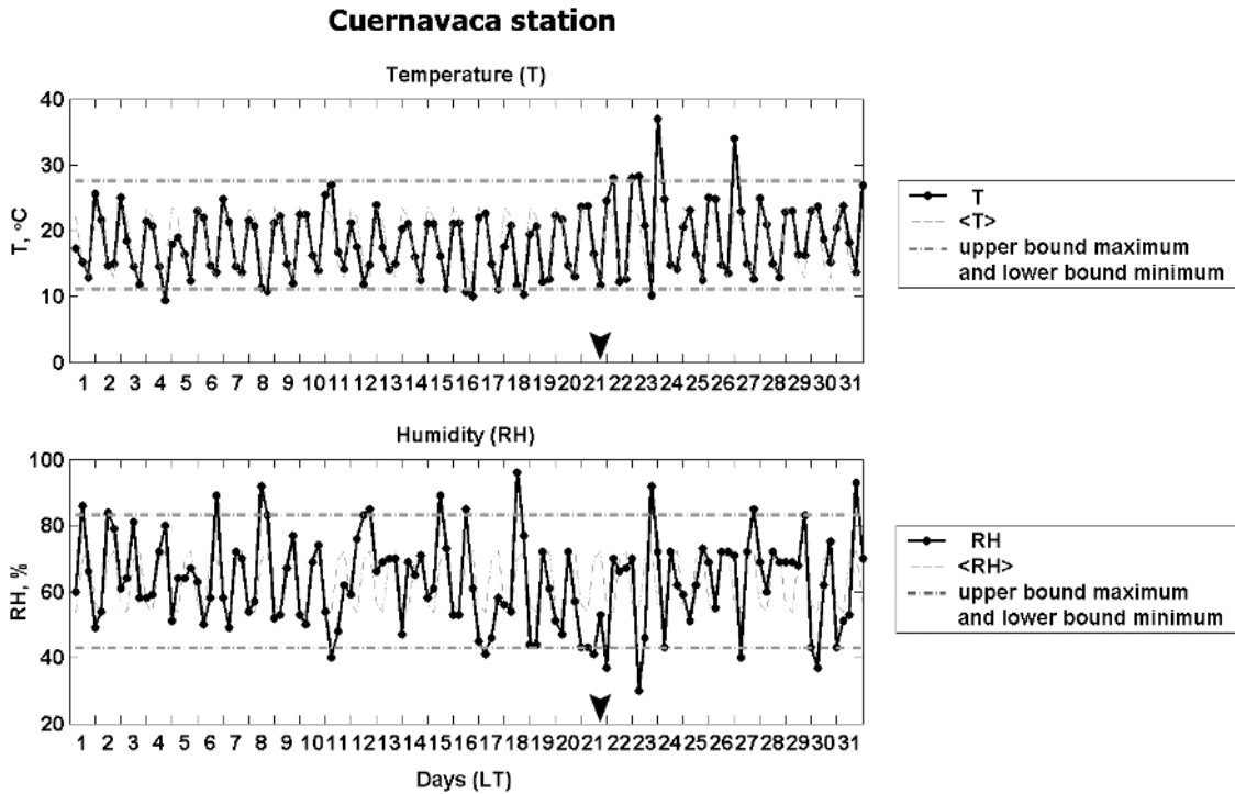
Fig. 4. Upper panel – ground air temperature at Cuernavaca station for January 2003, lower panel – relative humidity at the Cuernavaca station for January 2003. \nabla indicates the earthquake moment.
