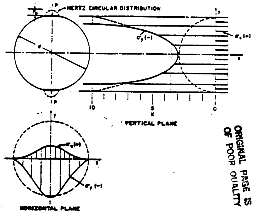
b Stress Distribution for Transversely Loaded Disk
