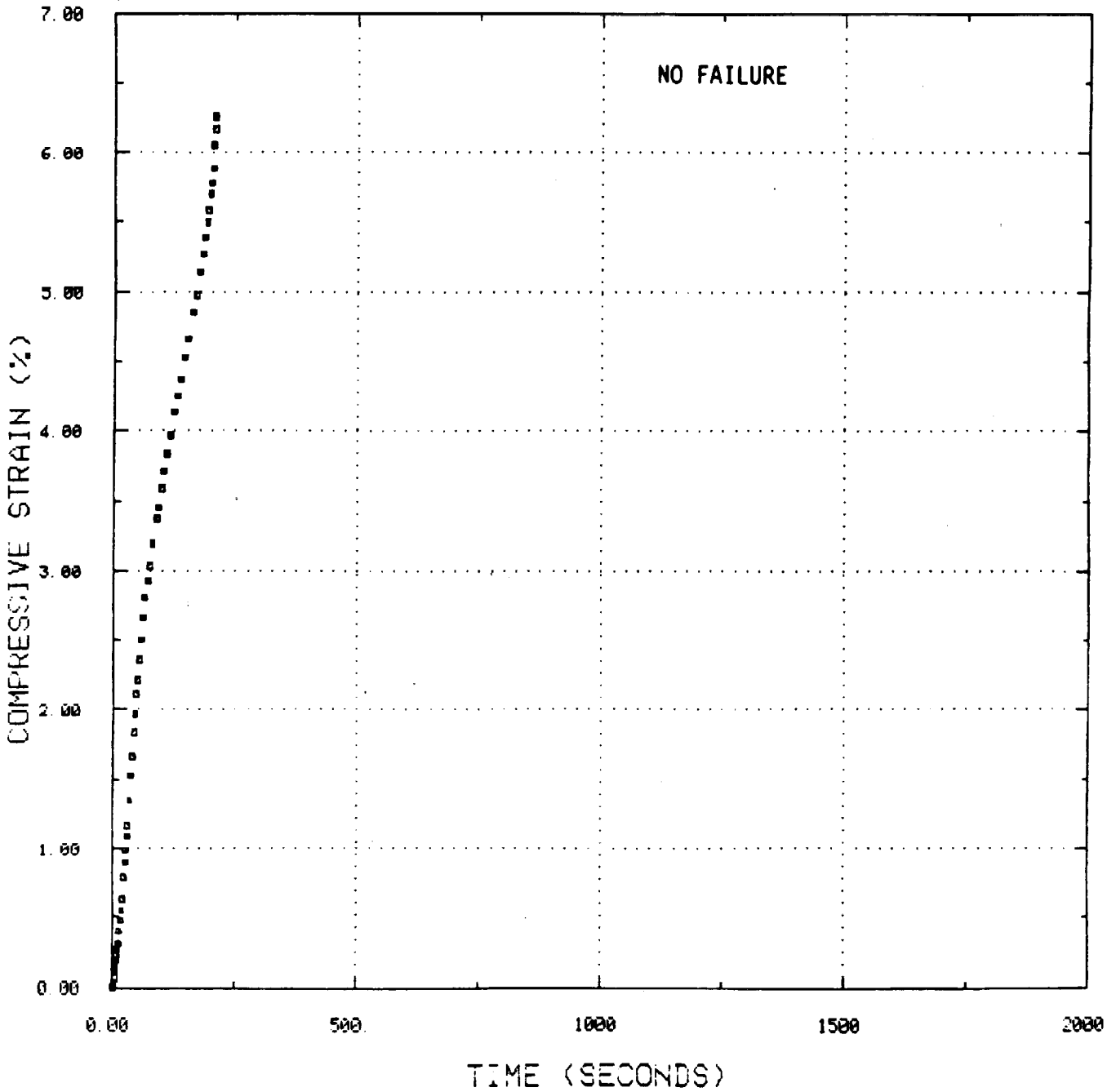
Figure E-23 Compression Creep Strain-Time (2200°F)
