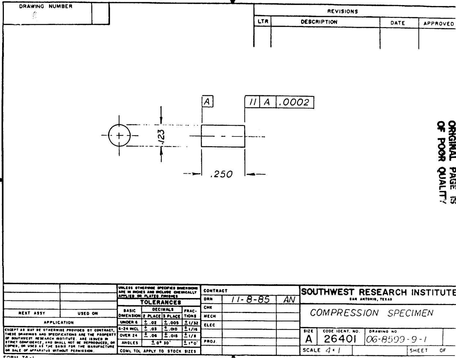
Figure 66 Compression Specimen
