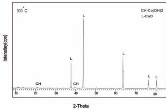
Figure 5. XRD pattern of calcite at 900 °C (sample TS2)
