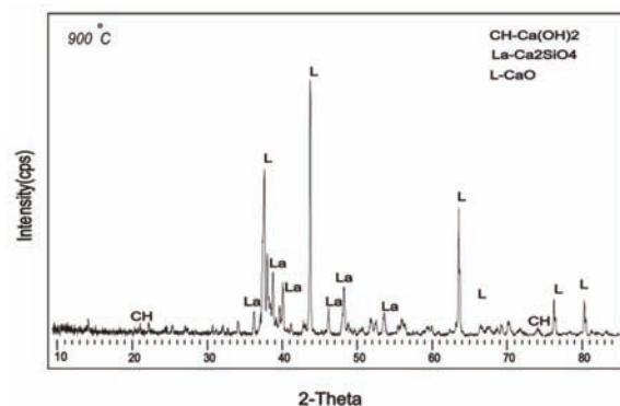
Figure 4. XRD pattern of calcite at 900 °C (sample TS1)
