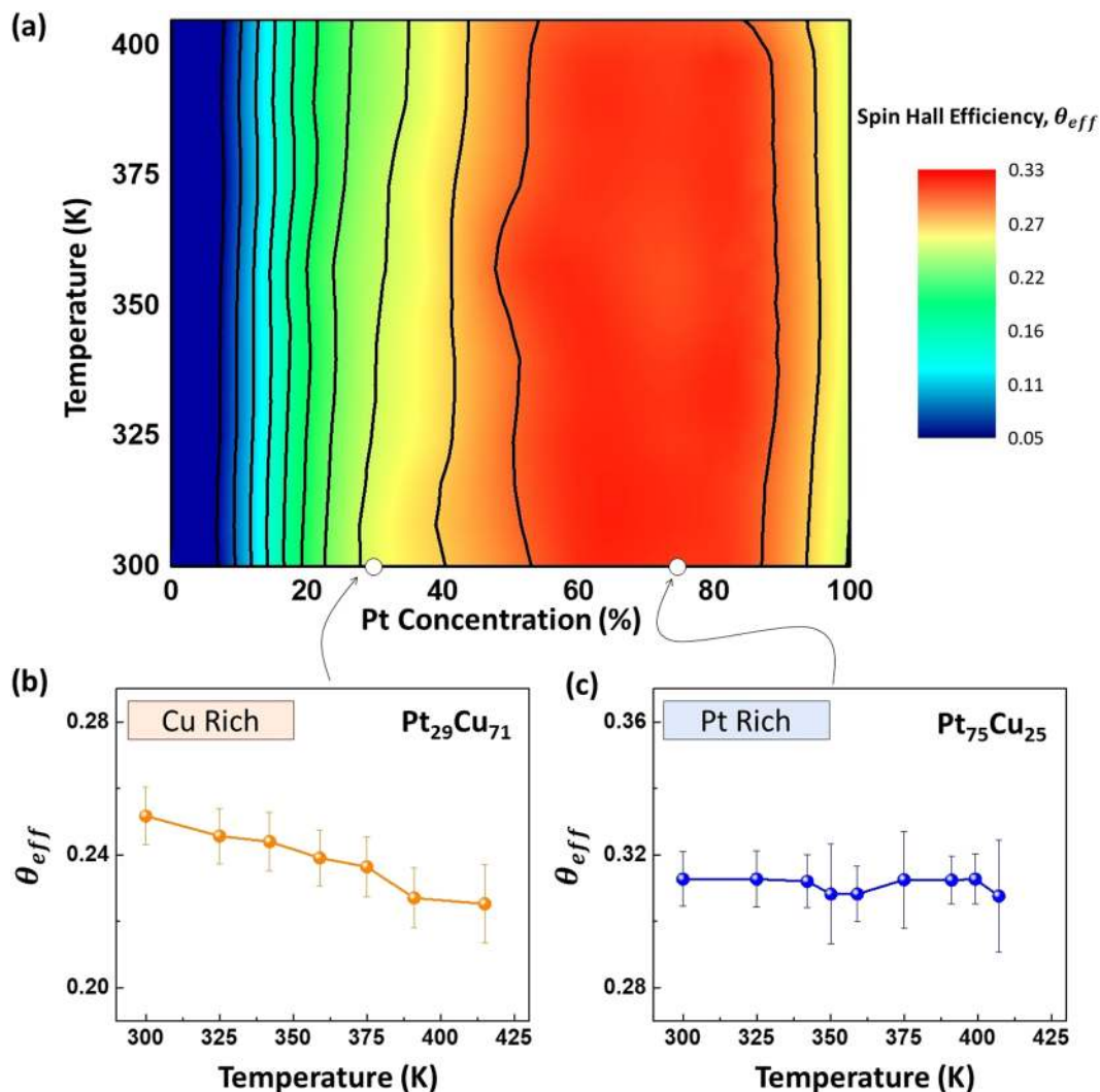
Figure 4. (a) Contour plot of \theta_{eff} for Pt_xCu_{1-x} (5 nm)/Co(5 nm)/Ta(5 nm) trilayer device with temperature for varying Pt concentrations. (b) and (c) Temperature dependence of \theta_{eff} for Cu-rich and Pt-rich Pt_xCu_{1-x} (5 nm)/Co(5 nm)/Ta(5 nm) trilayer device with x = 29\% and 75\% respectively.
