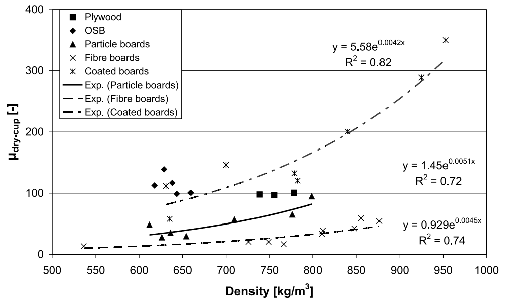
Fig. 4 Water vapour resistance factor ( \mu ) of the dry cup tests depending on the density (mean values)
