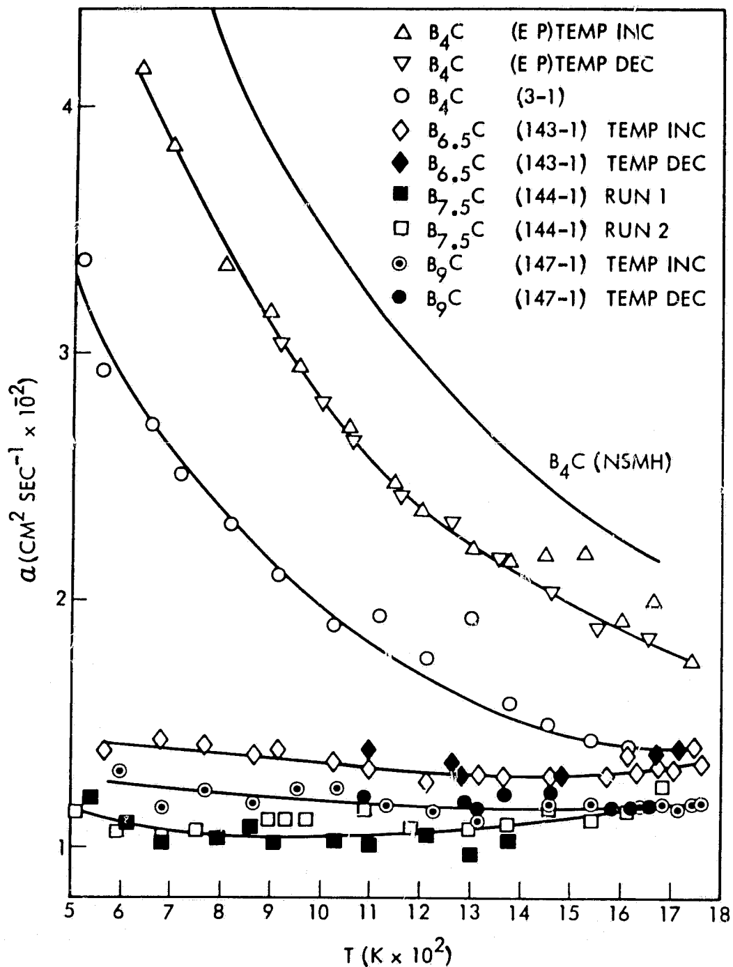
Fig. 1. The Thermal Diffusivity ( \alpha ) of Boron Carbides as a Function of Temperature (T) ([EP] refers to Eagle Picher Commercial Grade Boron Carbide and [NSMH] to Nuclear Systems Materials Handbook data 6 ).
