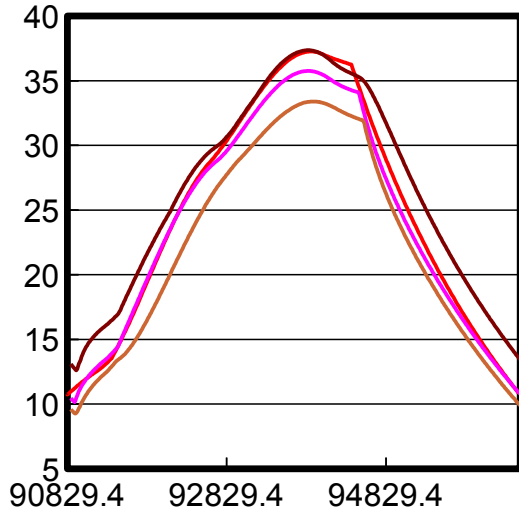
Figure 13. Comparison of temperature history at outer structure under worst hot case between two-nodal analysis with revised absorption at solar cells and multi-nodal analysis.
