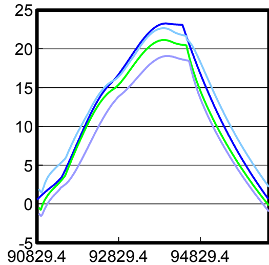
Figure 14. Comparison of temperature history at outer structure under worst cold case between two-nodal analysis with revised absorption at solar cells and multi-nodal analysis.
