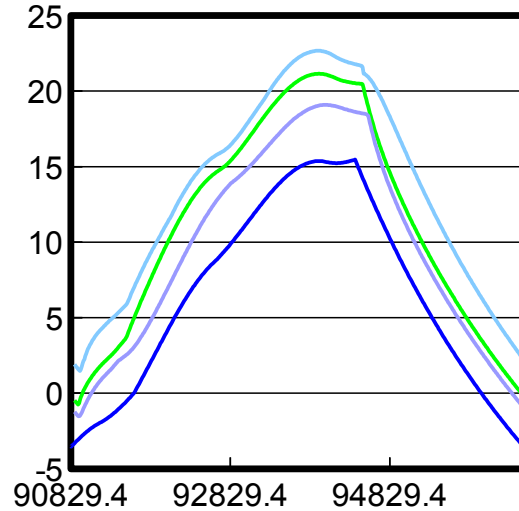
Figure 10. Comparison of temperature history at outer structure under worst cold case between two- and multi-nodal analyses.
