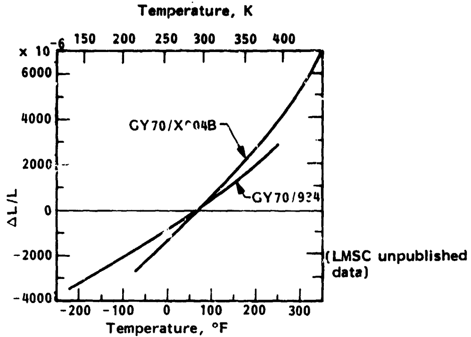
Figure 35. - Thermal expansion of GY70/X904B and GY70/934 unidirectional tape (90° fiber direction).
