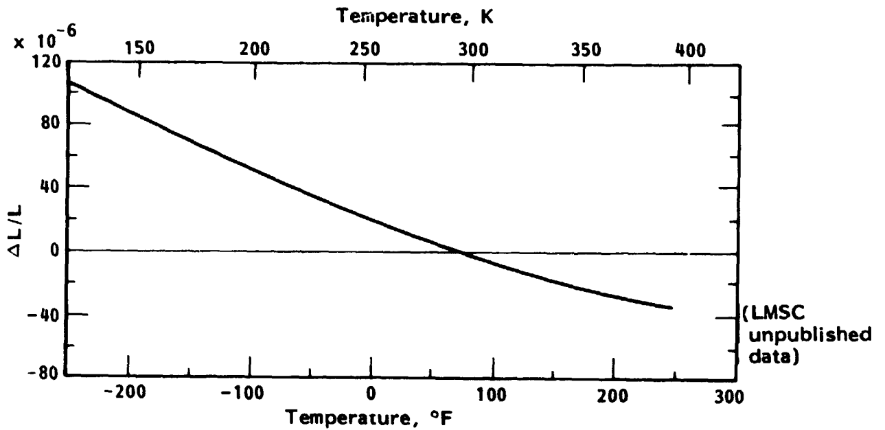
Figure 22. - Thermal expansion of unidirectional HMS/3501-5A tape (0° fiber direction).
