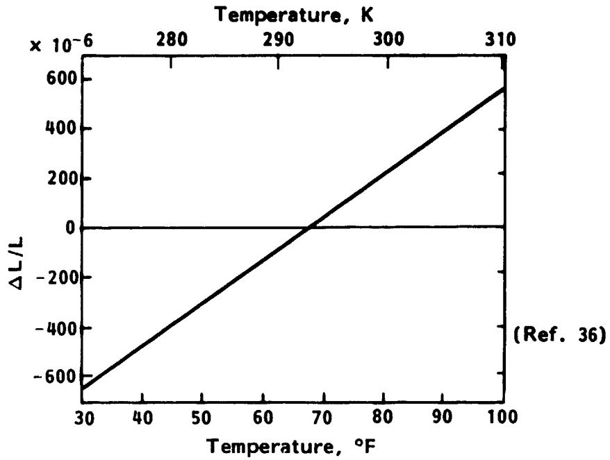
Figure 29. - Thermal expansion of HMS/759 unidirectional tape (90° direction).
