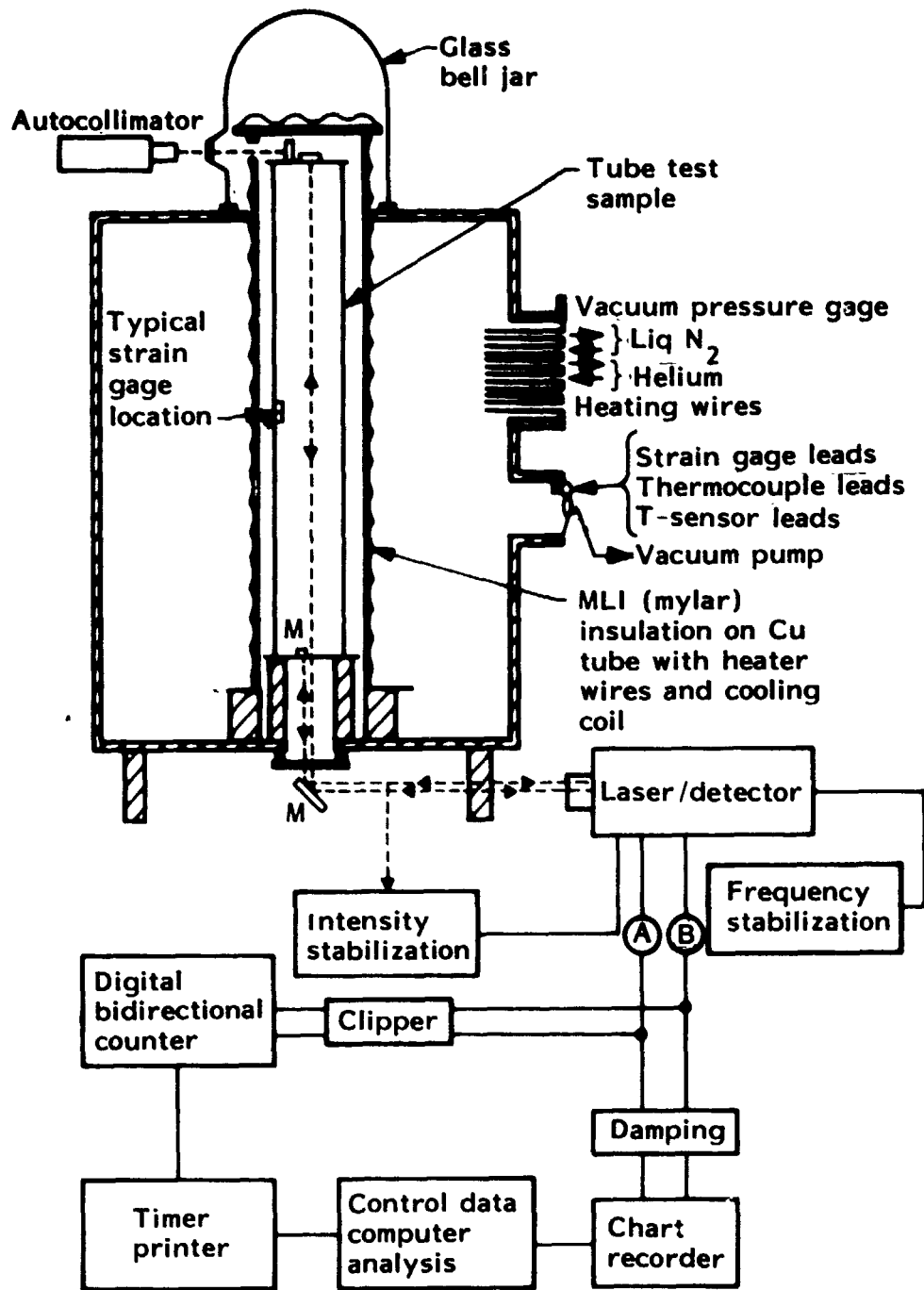
Figure 11. - Laser interferometer and dimensional stability test apparatus.
