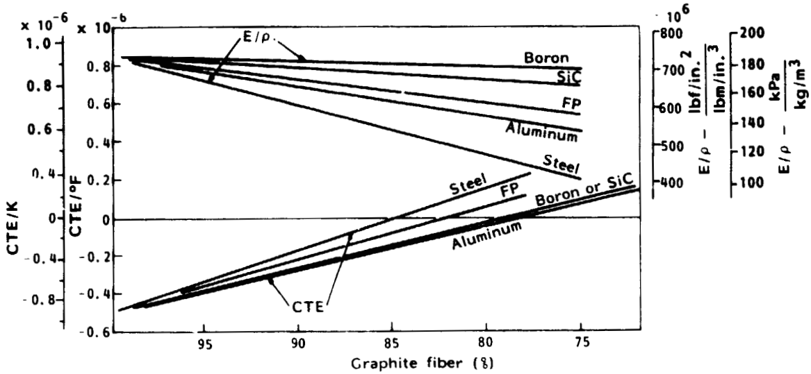
Figure 5. - Effect of replacing GY70 fiber with other selected fibers in a unidirectional laminate.
