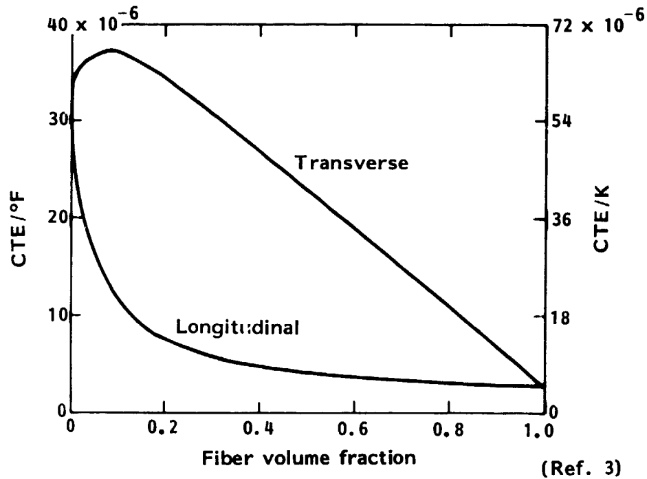
Figure 1. - Variation of CTE of a unidirectional glass fiber laminate with fiber volume.
