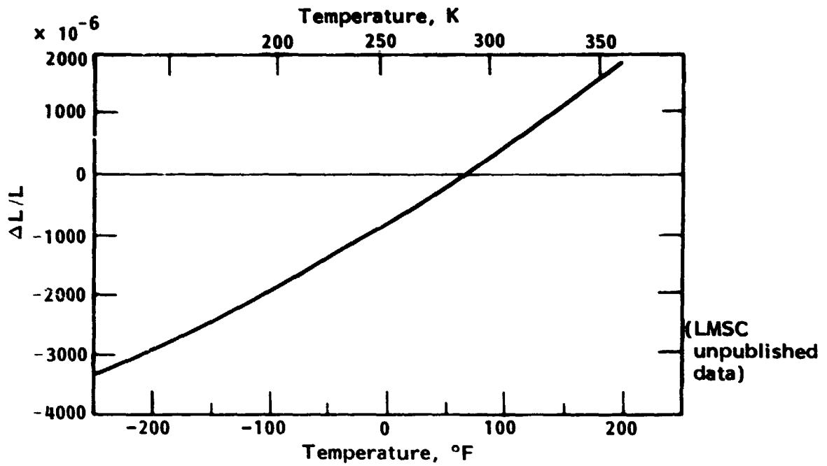
Figure 21. - Thermal expansion of unidirectional HTS-2/3501-5A tape (90° fiber direction).
