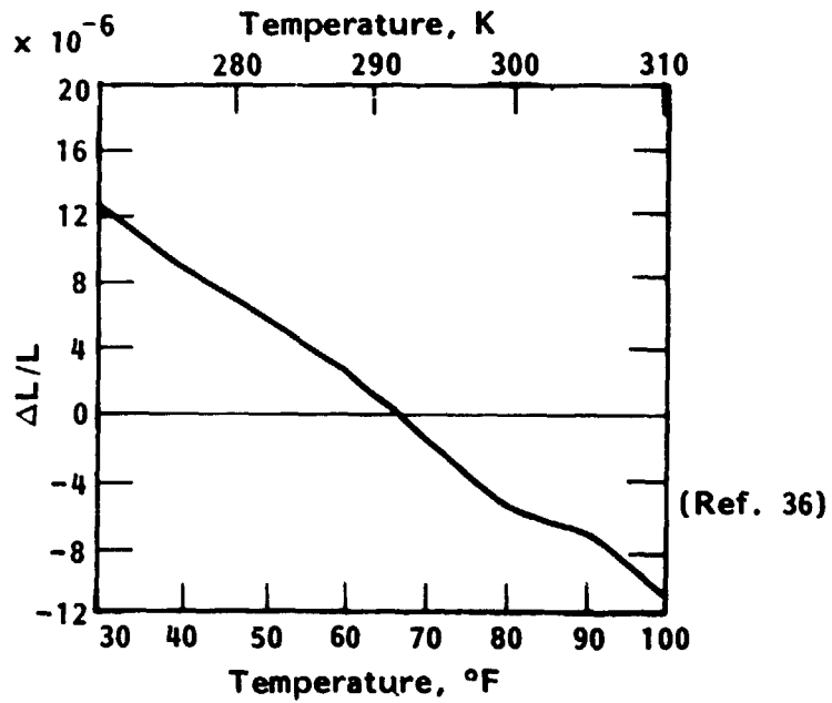
Figure 24. - Thermal expansion of HMS/3501 unidirectional tape (0° direction).
