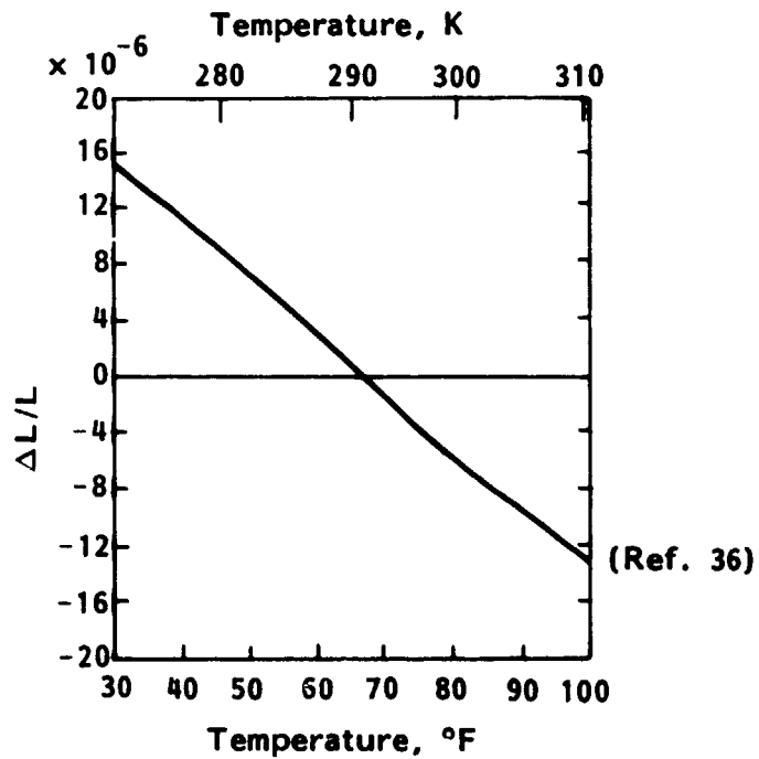
Figure 30. - Thermal expansion of HMS/934 unidirectional tape (0° fiber direction).
