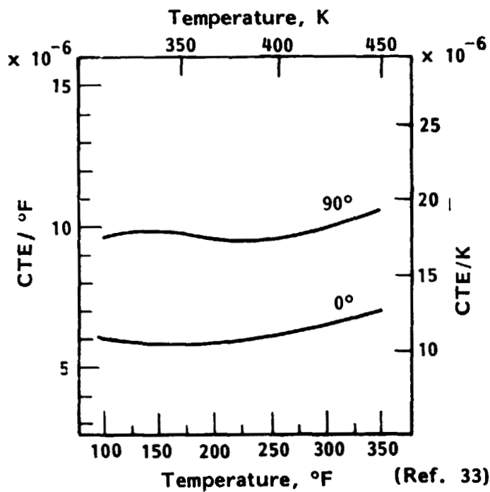
Figure 38. - Thermal expansion of 104 glass scrim cloth.
