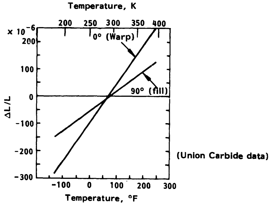
Figure 12. - Thermal expansion of Kevlar 49/X904B (120 style) fabric.
