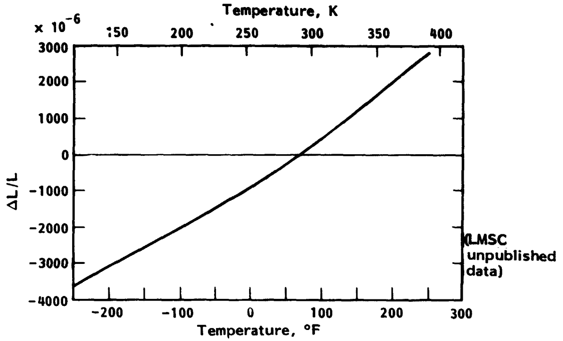
Figure 23. - Thermal expansion of unidirectional HMS/3501-5A tape (90° fiber direction).
