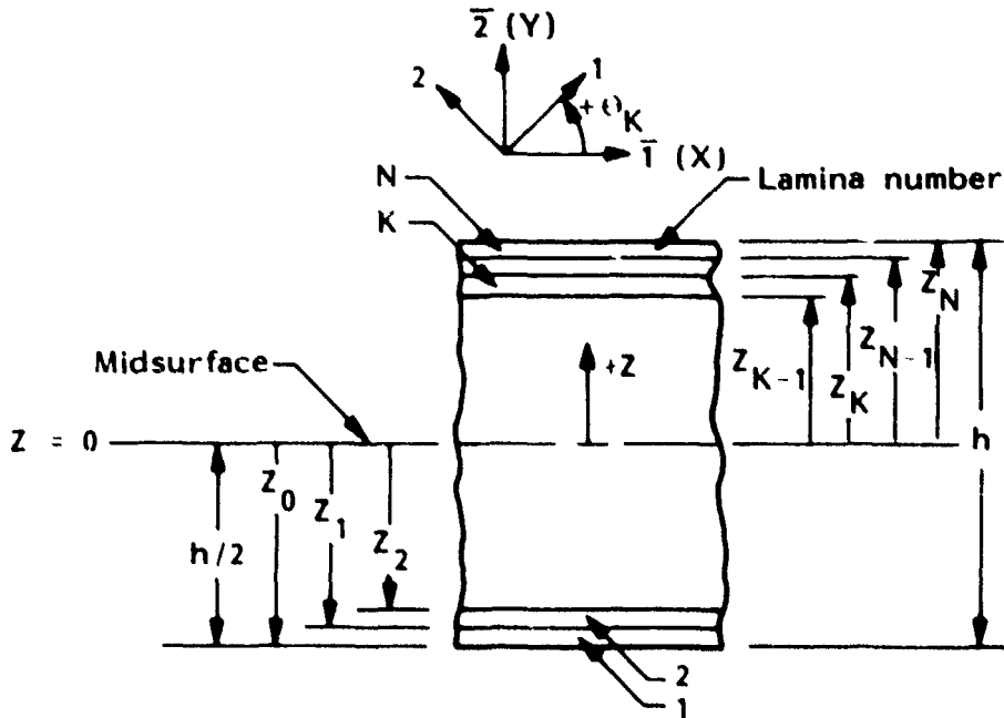
Figure 3. - Geometric representation of a laminate.
