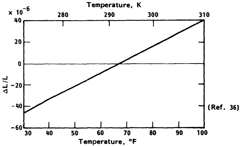
Figure 18. - Thermal expansion of HMF 330C/934 fabric (T-300 fiber) (0° warp direction).
