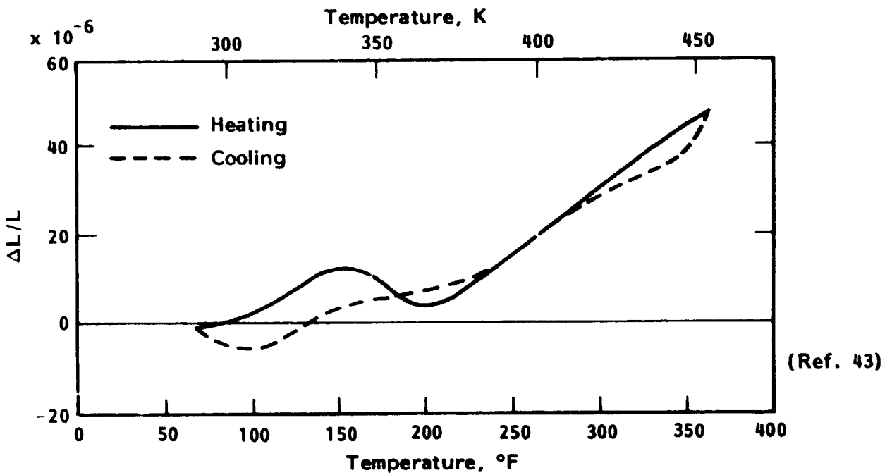
Figure 14. - Thermal expansion of Thornel 300/Narmco 5208 tape (0° fiber direction).
