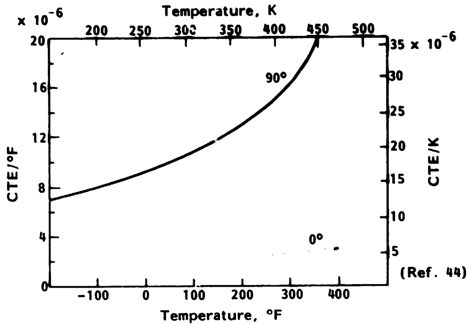
Figure 13. - Thermal expansion of unidirectional Boron/5505 tape.
