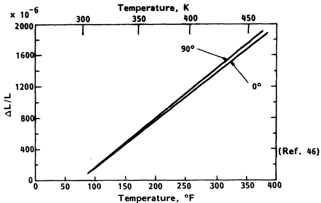
Figure 37. - Thermal expansion of glass/epoxy tooling material (181 cloth laminate).
