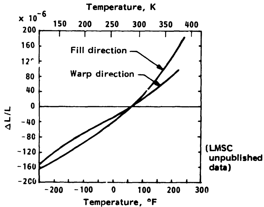
Figure 32. - Thermal expansion of HMS/E788 fabric.
