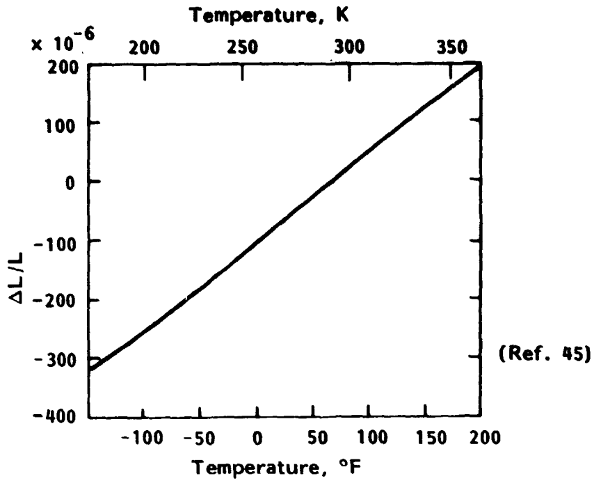
Figure 17. - Thermal expansion of HMF 330C/CE339 fabric (T-300 fiber) (90° fill direction).
