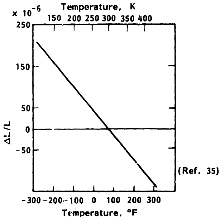
Figure 35. - Thermal expansion of GY70/X904B and GY70/934 unidirectional tape (90° fiber direction).
