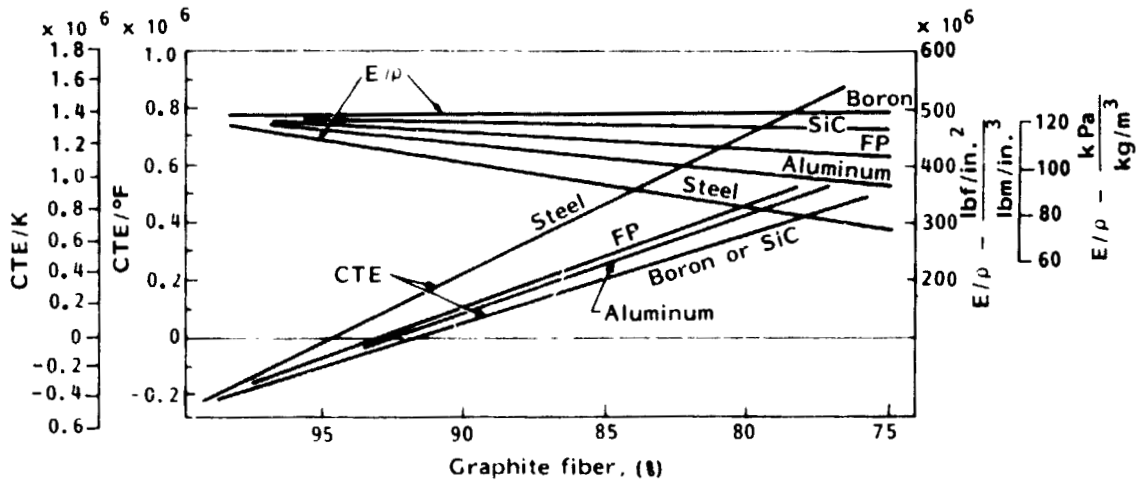
Figure 6. - Effect of replacing VSB-32 fiber with other selected fibers in a unidirectional layout.
