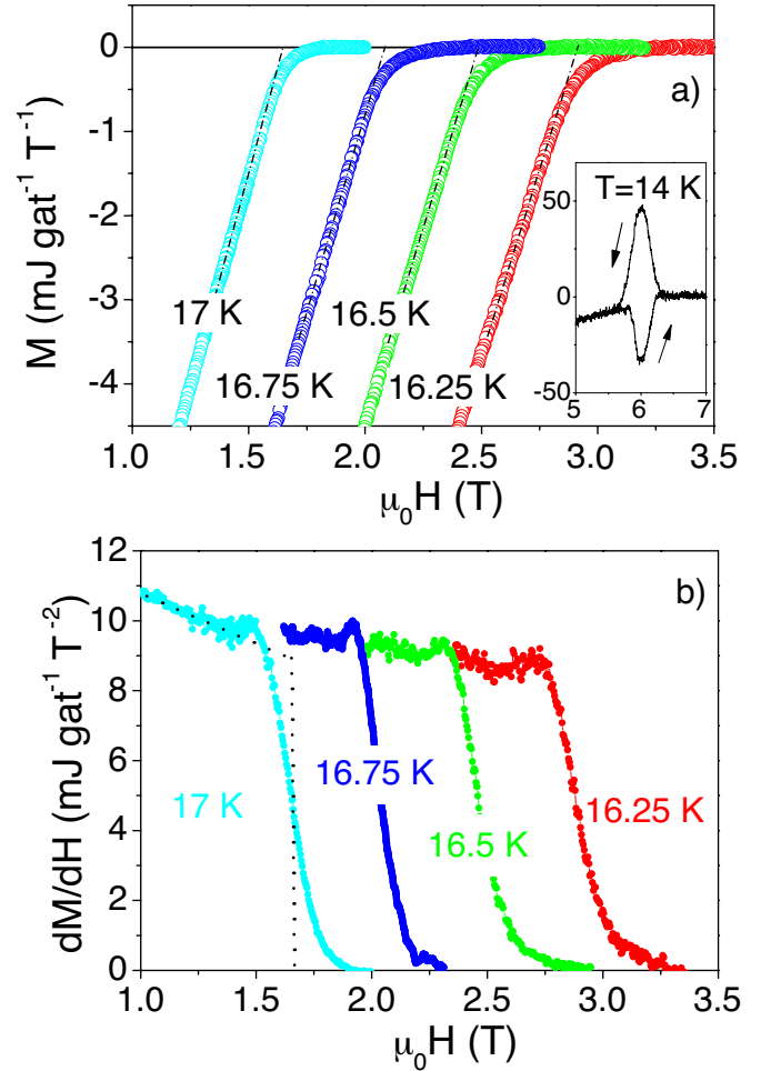
FIG. 2. (Color online) (a) Magnetization as a function of applied field at four different temperatures. The straight lines serve as a guide to the eye to show the deviation from linear behavior due to the onset of fluctuations close to T_c(H) . The inset shows a sharp hysteresis loop (“magnetization peak effect”) due to enhanced flux pinning at the lower onset of the fluctuation regime which develops at lower temperatures (here 14 K) (Refs. 17 and 18). (b) Derivative of the magnetization curves showing a small fluctuation peak superimposed on the broadened jump at T_c(H) . Consistent units \text{J gat}^{-1} \text{T}^{-1} = \text{Am}^2 \text{gat}^{-1} and \text{J gat}^{-1} \text{K}^{-1} are used for the magnetization and the specific heat respectively. Here 1 gat (gram-atom) is 1/4 mole.
