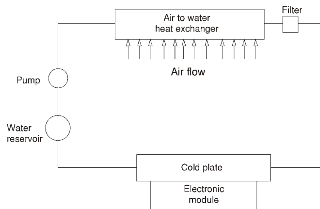
Figure 9. Indirect cooling of electronic module
