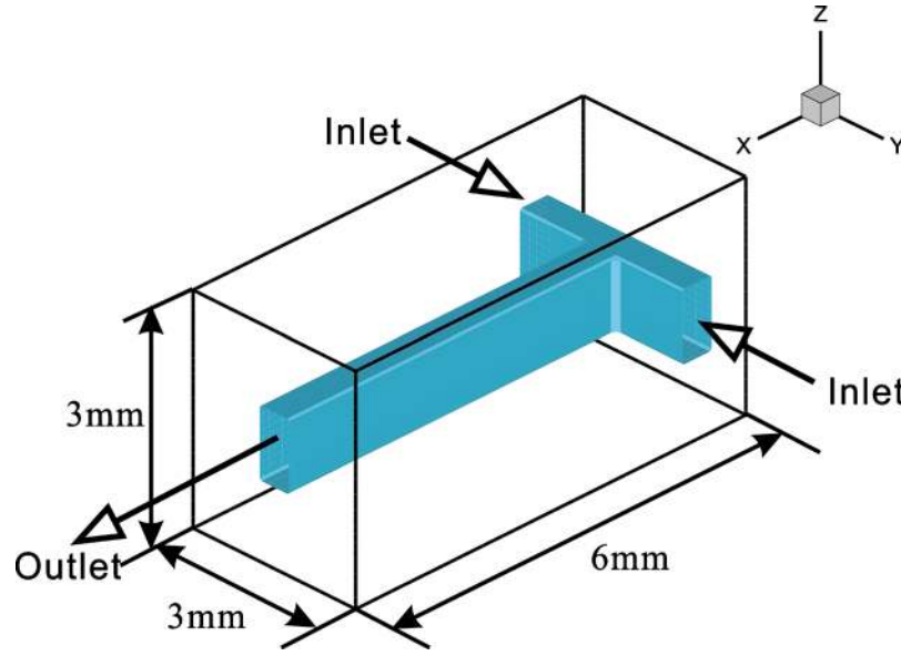
FIG. 8. Computational domain.
