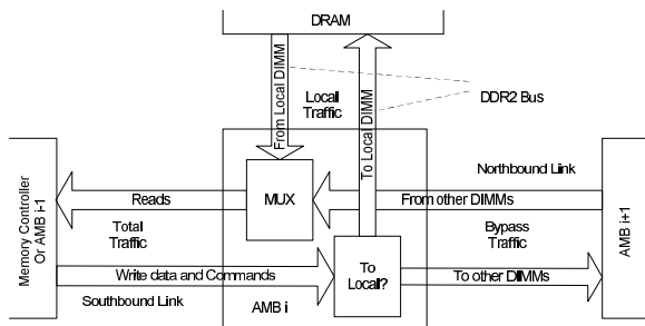
Figure 2: Four categories of data traffic that flows through AMB.
