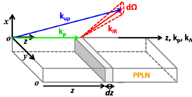
Fig. 3. Schematic diagram of the propagating wave vectors ( k_{\text{up}} , k_{\text{p}} , k_{\text{IR}} ) and the coordinate axes ( x , y , z ) used in the model. The pump beam and PPLN poling periodicity (wave vector is k_{\Lambda} ) is along the z -axis.
