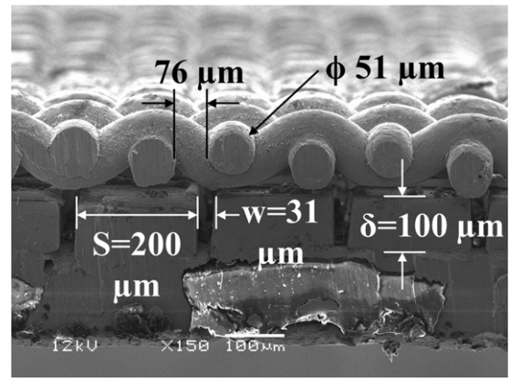
Figure 4. SEM image of the hybrid wicking structure consisting of a woven copper mesh bonded the top surface of 100 \mu\text{m} high electroplated copper pillars.
