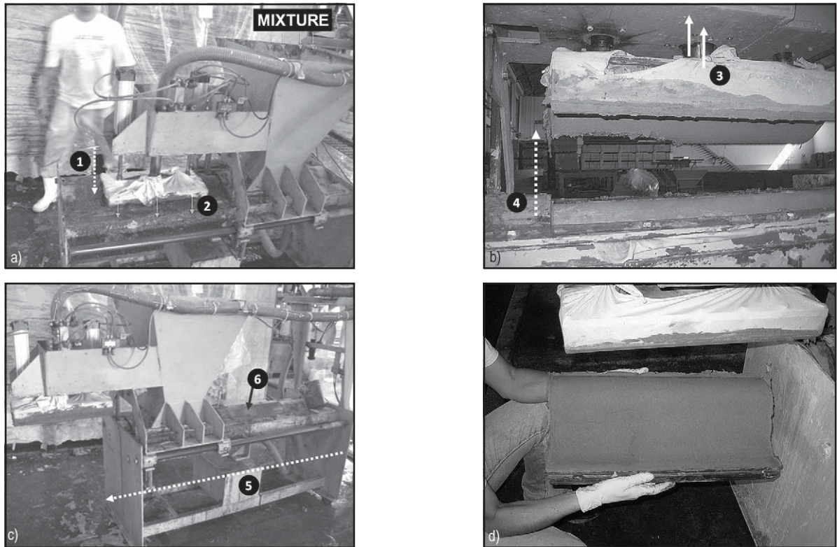
Figure 2 – Steps sequence of the automated device used for roofing tile molding: (a) pressing in the molding chamber (arrow 1) and dewatering (arrow 2); (b) suction by the upper device (arrow 3) and withdrawal from the molding chamber (arrow 4); (c) displacement of the upper device (arrow 5) and further filling the molding chamber with the mixture (arrow 6); (d) transfer of the tile to the undulate mold.
