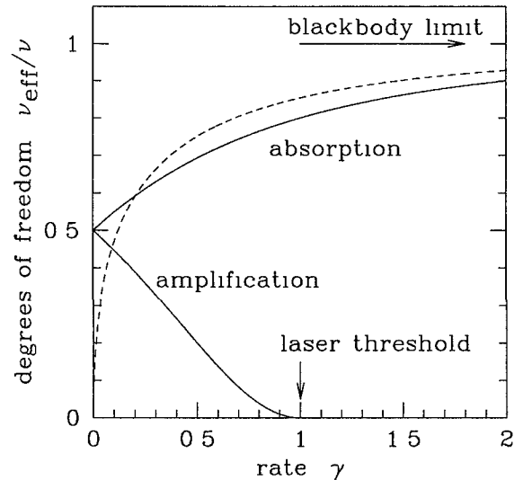
FIG 2 Effective number of degrees of freedom as a function of normalized absorption or amplification rate The dashed curve is for the disordered slab, the solid curves are for the chaotic cavity The amplifying slab would be above the laser threshold for any \gamma , so we only plot the case of absorption For the cavity, both cases of absorption and amplification are shown The blackbody limit for absorbing systems and the laser threshold for amplifying systems are indicated by arrows
