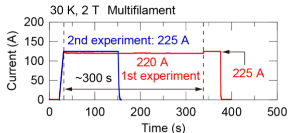
Fig. 17. Example of processes to determine the 300 s-thermal runaway currents in multifilament sample in thermal runaway detection and protection experiments (30 K, 2 T).
