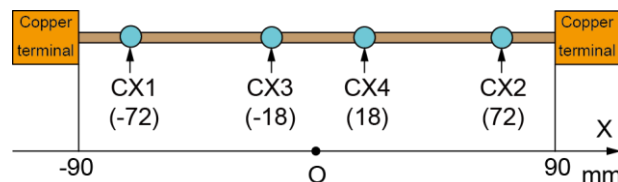
Fig. 4. Sample layout and positions of temperature sensors (CX i : Cernox temperature sensor). Numbers in blankets are relative positions to the longitudinal center of the short sample (unit: millimeter).
