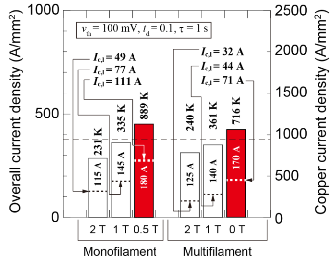
Fig. 20. Summary of the thermal runaway detection and protection experiments. White bar: after which no degradation was observed. Red bar: after which samples degraded. I_{c1} : critical current at local defect measured between a5 and a6 in monofilament sample, and between a3 and a4 in multifilament sample (length: 20 mm, electric field: 100 \mu\text{V/m} ).
