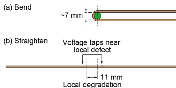
Fig. 16. Side view of sample with local defect (by bending). (a) Bending sample to create a local and uniform defect across its width (~11 mm length). (b) Straightened sample.
