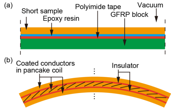
Fig. 13. Construction of short samples and coated conductors in pancake coil across their thicknesses. (a) Short sample. (b) Coated conductors in middle turns of pancake coil.
