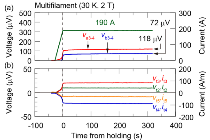
Fig. 10. Example of voltages and currents of multifilament sample with local defect at 190 A, 30 K, 2 T (no thermal runaway initiated in 300 s). (a) Voltages on longitudinal direction. (b) Voltages and currents on transverse direction (after the current reached 190 A in Fig. 8(b), 1st experiment; v_{am-n} : voltage between tap am and an ; v_{bm-n} : voltage between tap bm and bn ; v_{i/i} : voltage/current between tap ai and bi ).
