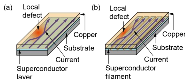
Fig. 3. Current distribution in the coated conductor with local defect. (a) Monofilament coated conductor. (b) Multifilament coated conductor.
