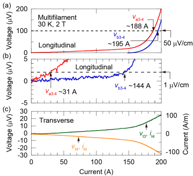
Fig. 7. Voltage-current characteristics of multifilament sample with local defect at 30 K, 2 T. (a) Voltages on longitudinal direction. (b) Voltages on longitudinal direction (enlarged). (c) Voltages/currents on transverse direction. ( v_{am-n} : voltage between tap am and an ; v_{bm-n} : voltage between tap bm and bn ; v_{i/i} : voltage/current between tap ai and bi ).
