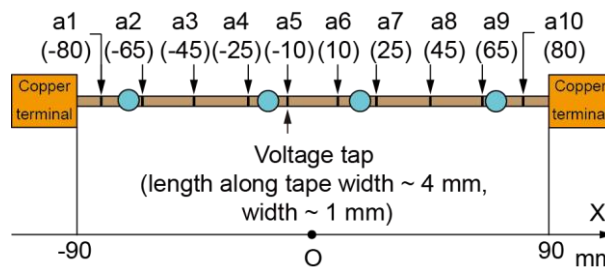
Fig. 15. Positions and geometry of voltage taps of monofilament sample in thermal runaway detection and protection experiments (ai: voltage tap). Numbers in blankets are relative positions to the longitudinal center of the short sample (unit: millimeter).
