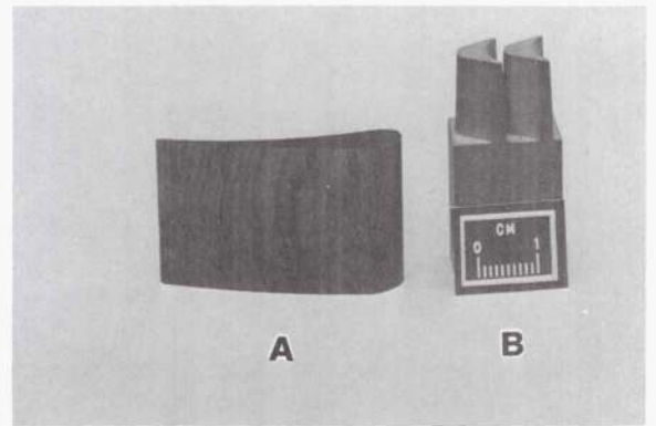
FIGURE 4. - FIBER REINFORCED CERAMIC MATRIX COMPOSITE TURBINE BLADES.
