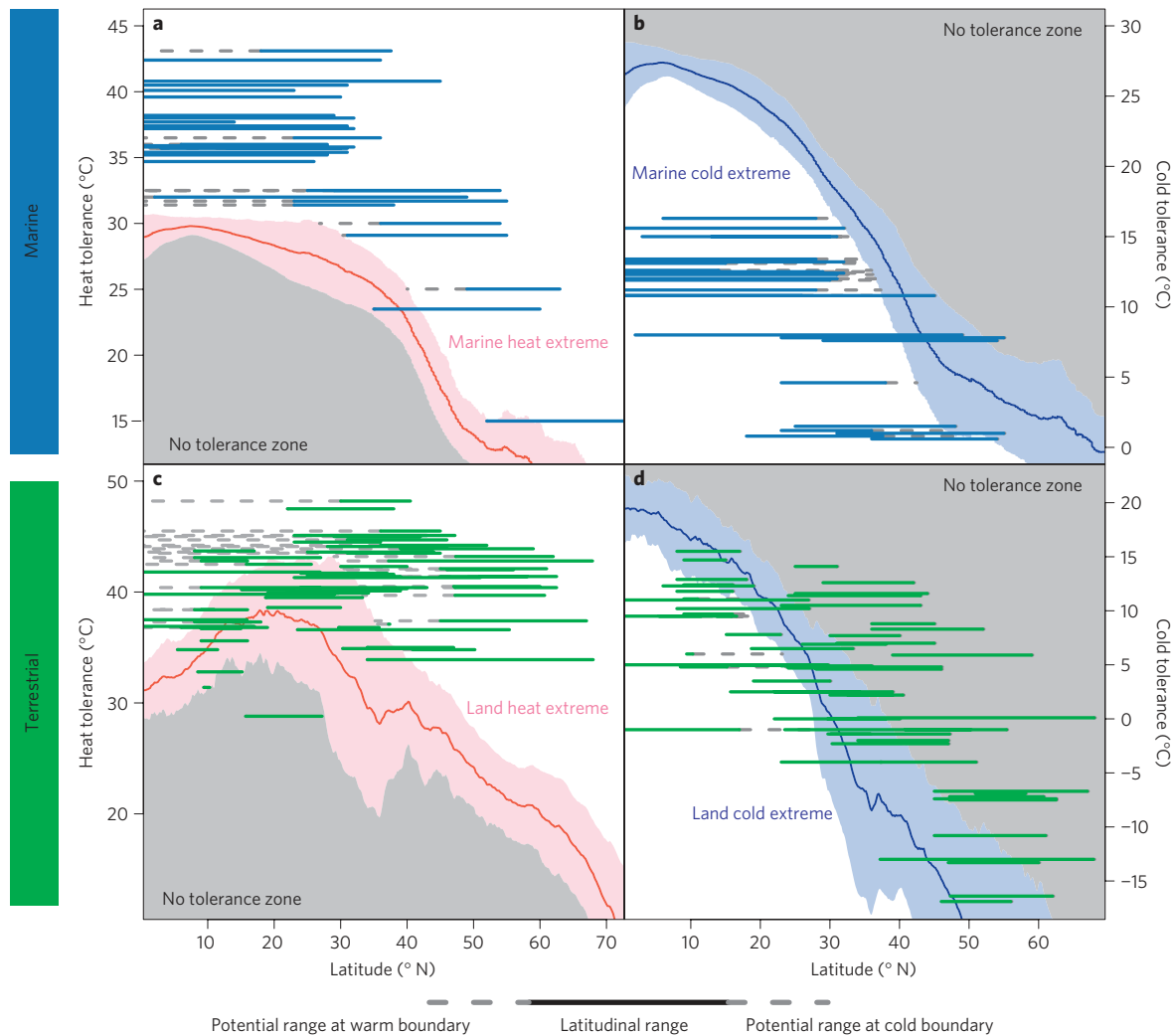
Figure 2 | Potential and realized latitudinal range boundaries of ectotherms. a–d, The realized latitudinal ranges of marine (a,b) and terrestrial (c,d) ectotherms represented as solid horizontal bars along the x axis, versus species' heat (a,c) and cold (b,d) tolerance limits on the y axis. The mean temperature of the warmest (red) or coldest (blue) month for each latitude from long-term climate data is shown, with shaded regions showing standard deviation across longitude. Grey shaded regions show where species' critical thermal tolerance would be insufficient to remain active in extreme warm (a,c) and cold (b,d) temperatures. Dashed grey horizontal lines show the extent of latitudes that species could potentially occupy on the basis of thermal tolerance alone.
