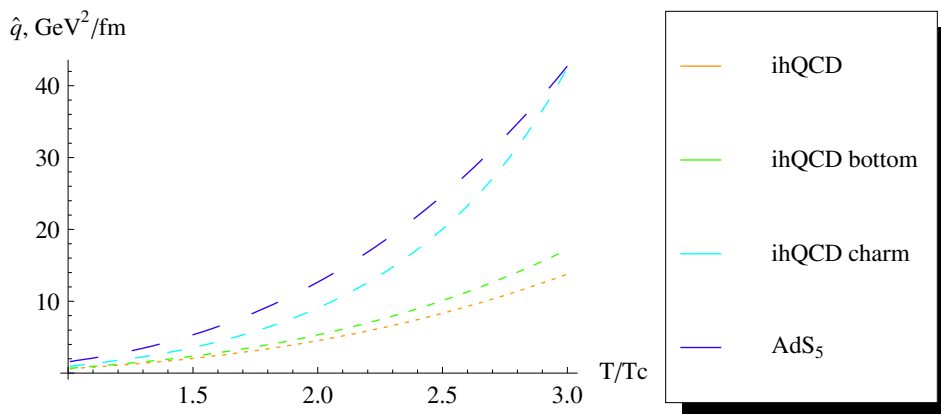
Figure 17. The jet quenching parameter \hat{q} for the Improved Holographic QCD model and \mathcal{N} = 4 SYM is shown in units of GeV^2/fm for a region close to T = T_c . The smallest dashed curve is the ihQCD result with an effective cutoff of r_{\text{cutoff}} = r_h/1000 . The small dashed curve is the ihQCD result with the cutoff from the mass of the Bottom quark. The medium dashed curve has a cutoff coming from the Charm mass and and largest dashed curve is the \mathcal{N} = 4 SYM result.
