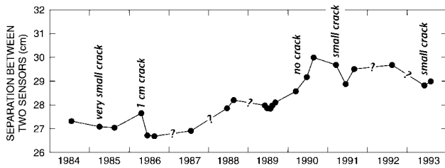
FIGURE 31. The 1984 to 1993 changes in separation for the two free-floating sensors (#14 and #5) shown in Figure 30. See text.
