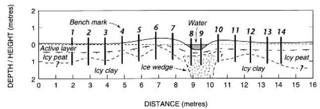
FIGURE 23. Vertical cross section from near BM 1 in the centre of Polygon A to BM 14 in the centre of Polygon B (see Fig. 20).
