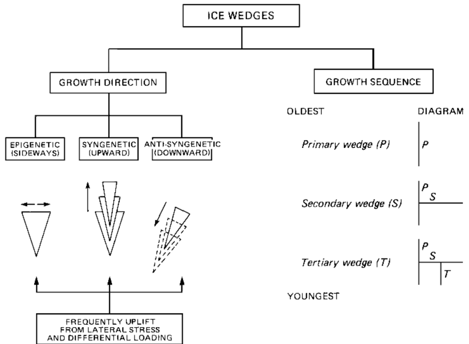
FIGURE 2. Classification system for ice wedges that is based upon the growth direction and growth sequence. The ice wedges are shown in cross sections in vertical profiles. An epigenetic wedge grows in a stable area where the growth is in width but not in height; a syngenetic wedge grows progressively upward at a site of permafrost aggradation; and an anti-syngenetic wedge grows downward at a site where there is removal of material, as by mass wasting. The growth sequence, shown in plan view, is from primary to tertiary wedges.
