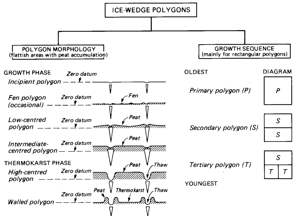
FIGURE 3. Classification system for ice-wedge polygons in flattish areas. The wedges are shown in cross sections in vertical profiles. The growth normally progresses from an incipient polygon to an intermediate centred polygon. The thermokarst phase has been subdivided, for simplicity, into high-centred polygons and walled polygons. The growth sequence, shown in plan view, is from primary polygons, which are often rectangular in homogeneous flattish areas, to tertiary polygons.
