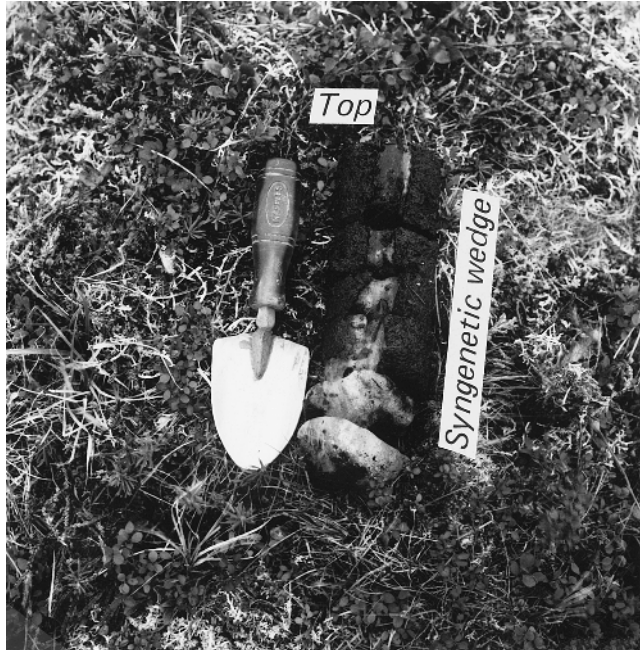
FIGURE 34. Drill core collected at the drilling site of Figure 33 showing the top of a narrow syngenetic wedge that propagated upward from the epigenetic wedge at the bottom. The 20 cm long trowel provides scale.
