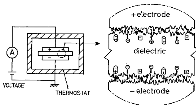
Figure 2. Illustration of the injection of homocharges \oplus . The internal heterocharging by dipole orientation \odot and ion migration \square is also shown.
