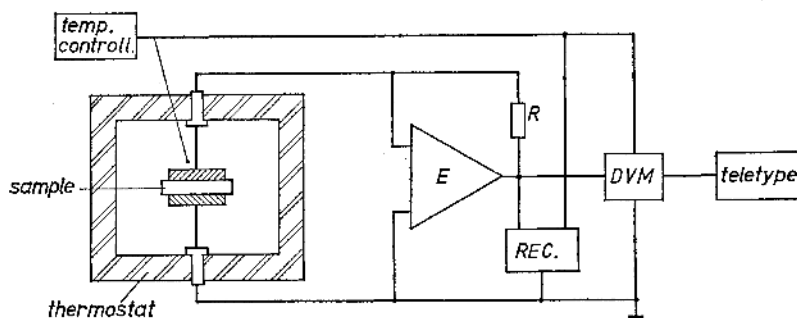
Figure 6. Set-up for automatic TSD measurements.
