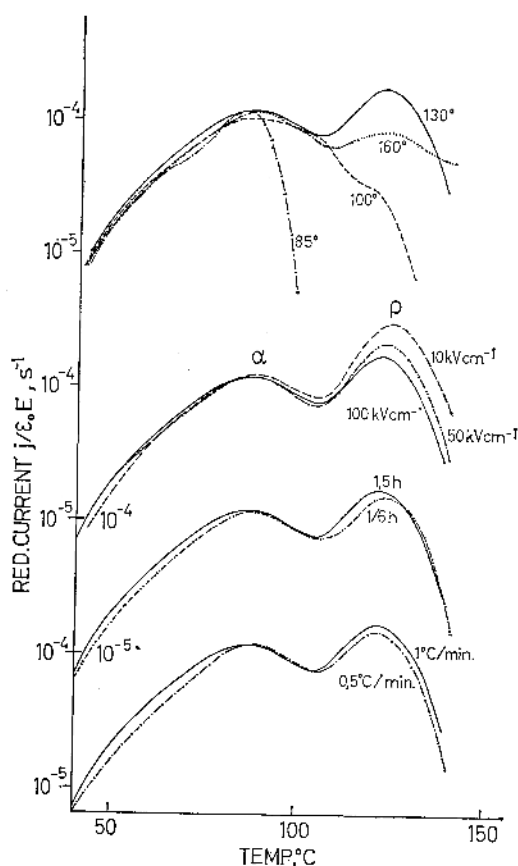
Figure 12. Results of PET electrets formed under different conditions; heating rate, 0.5^{\circ}\text{C/min} .
