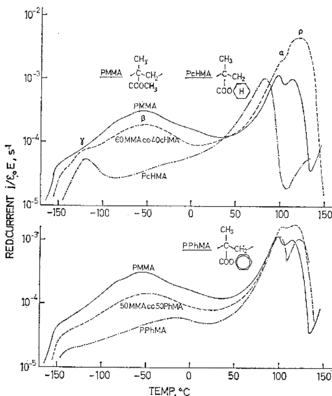
Figure 10. TSD of methacrylic homo- and copolymers with cyclic alkyl side groups.
