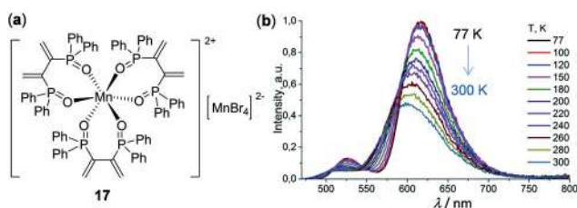
Fig. 16 (a) Molecular structure of Mn(II) complex 17 . (b) Temperature-dependent solid-state emission spectra of 17 under excitation at 440 nm in the range of 77–300 K. Reprinted with permission from ref. 105a. Copyright 2018 The Royal Society of Chemistry.
