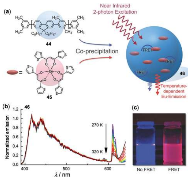
Fig. 35 (a) Molecular structures of 44 and 45 and schematic illustration showing the mechanism of the FRET-based nano-thermometer of the binary-assembled composite 46. (b) Normalized temperature-dependent emission spectra of 46 with two-photon excitation ( \lambda_{\text{ex}} = 720 \text{ nm} ). (c) Photographs exhibiting the emission color change of the nano-particles before (left) and after precipitation (right) in water under UV irradiation. Reprinted with permission from ref. 147. Copyright 2016 WILEY-VCH.
