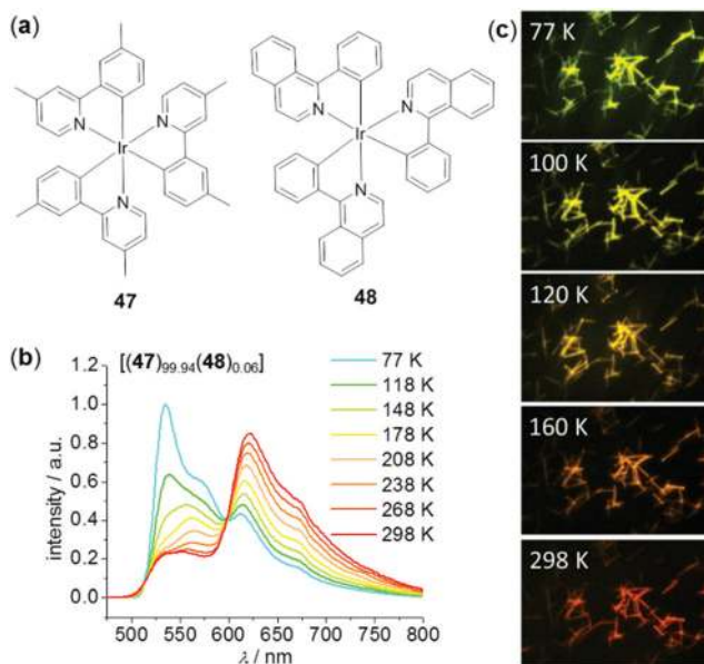
Fig. 36 (a) Molecular structures of donor 47 and acceptor 48. (b) Temperature-dependent emission spectra of nanotube 47 doped with 0.06% of 48 ( \lambda_{\text{ex}} = 375 \text{ nm} ). (c) Fluorescence microscopy images displaying the temperature-dependent emission color changes of the doped nanotubes. Reprinted with permission from ref. 149. Copyright 2018 Wiley-VCH.
