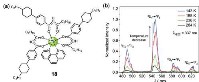
Fig. 17 (a) Molecular structure of Tb(III) complex 18 . (b) Temperature-dependent time-delayed emission spectra of a film with a time delay of 2.5 \mu\text{s} . Reprinted with permission from ref. 107. Copyright 2018 The Royal Society of Chemistry.
