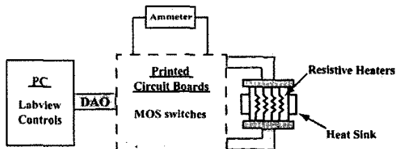
Figure 2. Experimental layout showing the fabricated device on top of heat sink at the right, the switching and measurement electronics in the center, and the computer with the digital-to-analog boards at the left.
