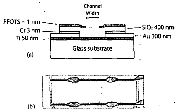
Figure 1. (a) Cross-section of completed thermocapillary actuation device. Maximum power dissipation occurs in the center region of the titanium layer where both Cr and Au have been removed. The lower surface energy of the PFOTS monolayer serves to confine liquids over the microheater and defines the width of each droplet. Card edge connectors contact the Au film at both ends. (b) Top-view of a single microheater (heater width 3 mm). Constrictions in the heater slightly increase local resistive power dissipation and help center the drops (Note: contact leads are not shown).
