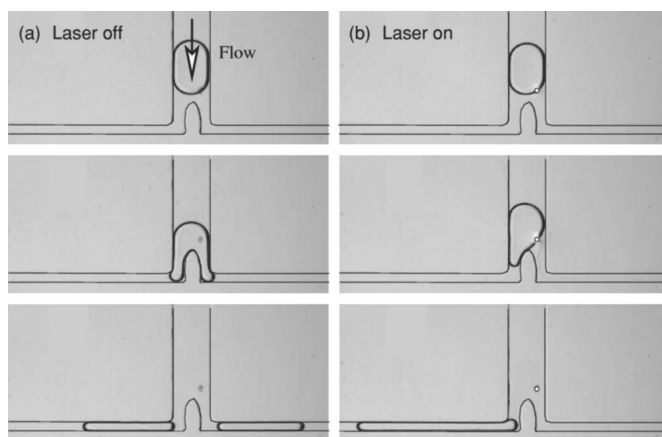
FIG. 4. Sorting drops: (a) Without laser forcing, a drop at a bifurcation divides into approximately equal daughter droplets. (b) When the laser forcing is applied, the drop advance in the right-hand channel is blocked so the whole drop is diverted into the left channel. Main channel width is 200\ \mu\text{m} and the operating conditions are Q_{\text{water}}=0.02\ \mu\text{L}/\text{min} , Q_{\text{oil}}=0.2\ \mu\text{L}/\text{min} , and \omega_0=5.2\ \mu\text{m} .
