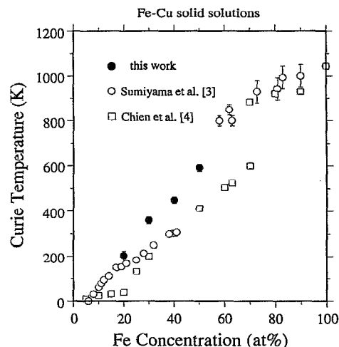
FIG. 7. Curie temperature, T_c , vs x for ball milled Fe-Cu fcc solid solutions (filled circles). Data for vapor deposited fcc and bcc solutions from the literature 3,4 have been included for comparison.
