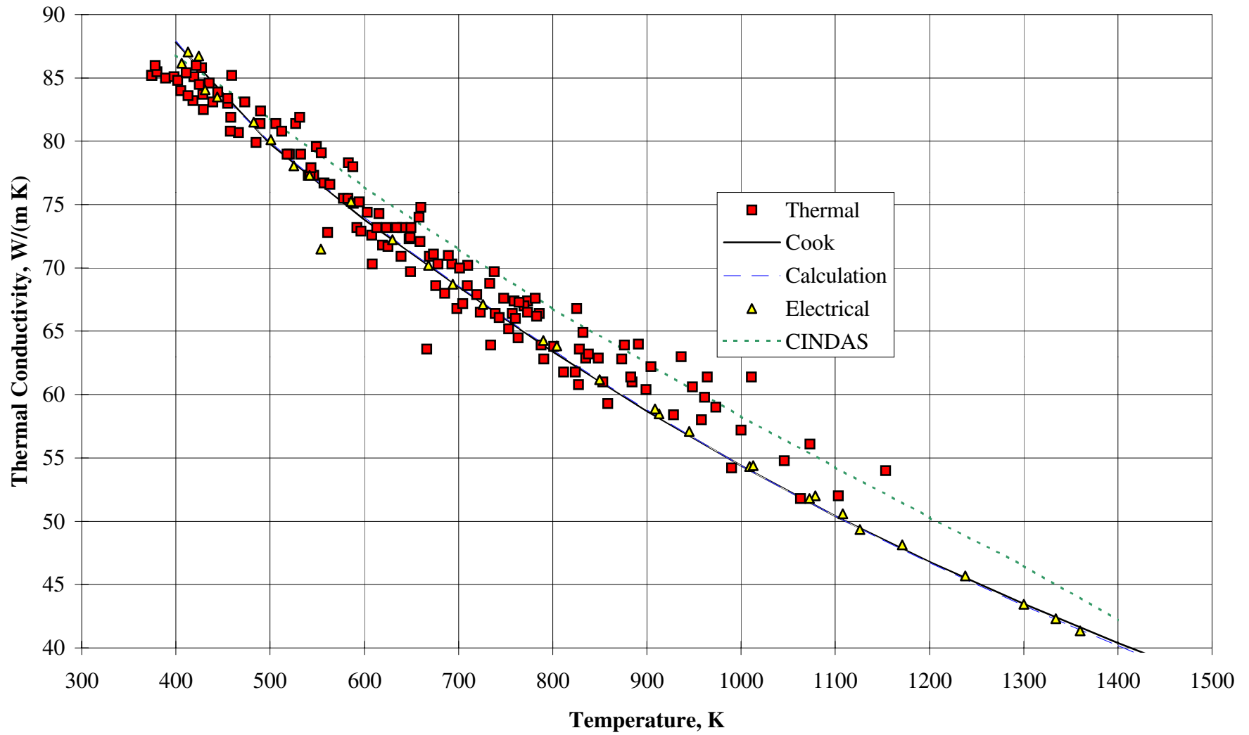
Fig 2.1-5 Comparison of Data from Thermal Conductivity Measurements and Resistivity Data Converted to Conductivity using Eq.(6) with Values from Cook and Fritsch, CINDAS, and the Calculation in this Assessment
