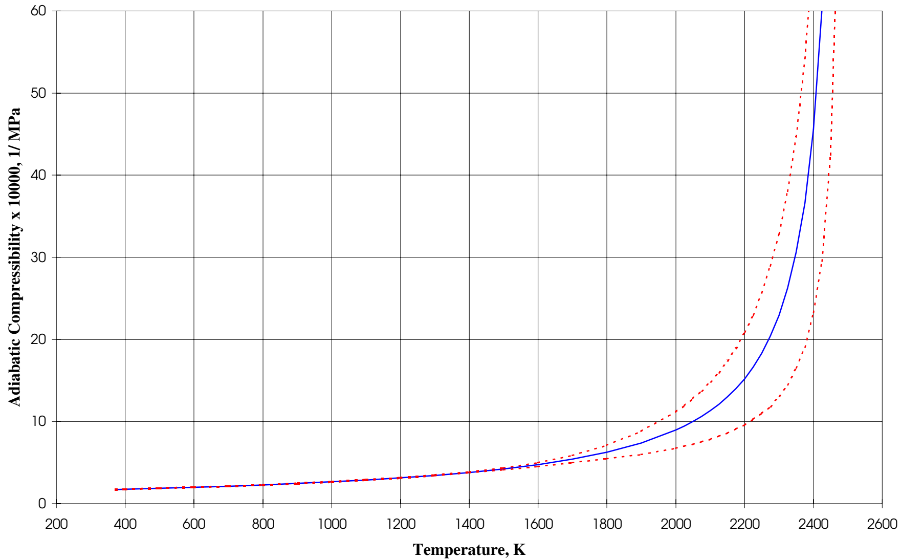
Fig. 1.4-1 Recommended Values for the Adiabatic Compressibility of Liquid Sodium
