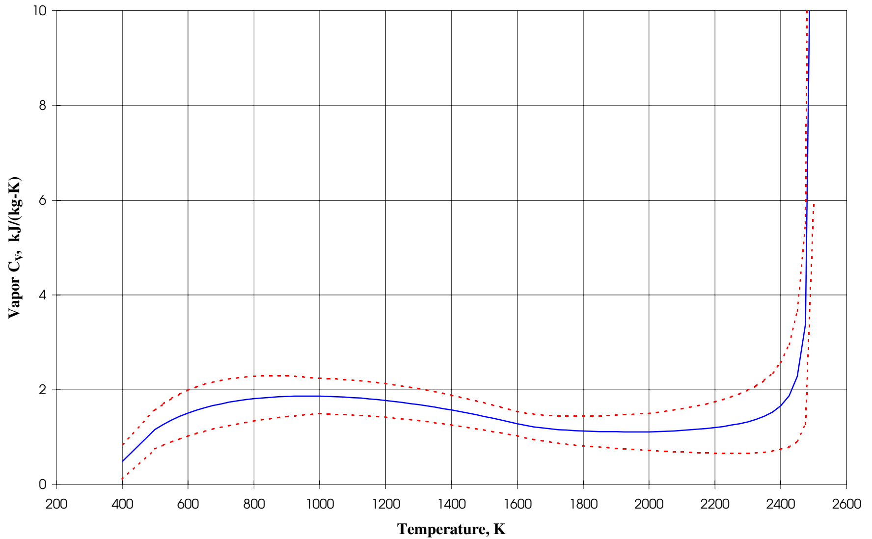
Fig. 1.1-23 The Heat Capacity at Constant Volume for Sodium Vapor with Estimated Uncertainties (dotted lines)
