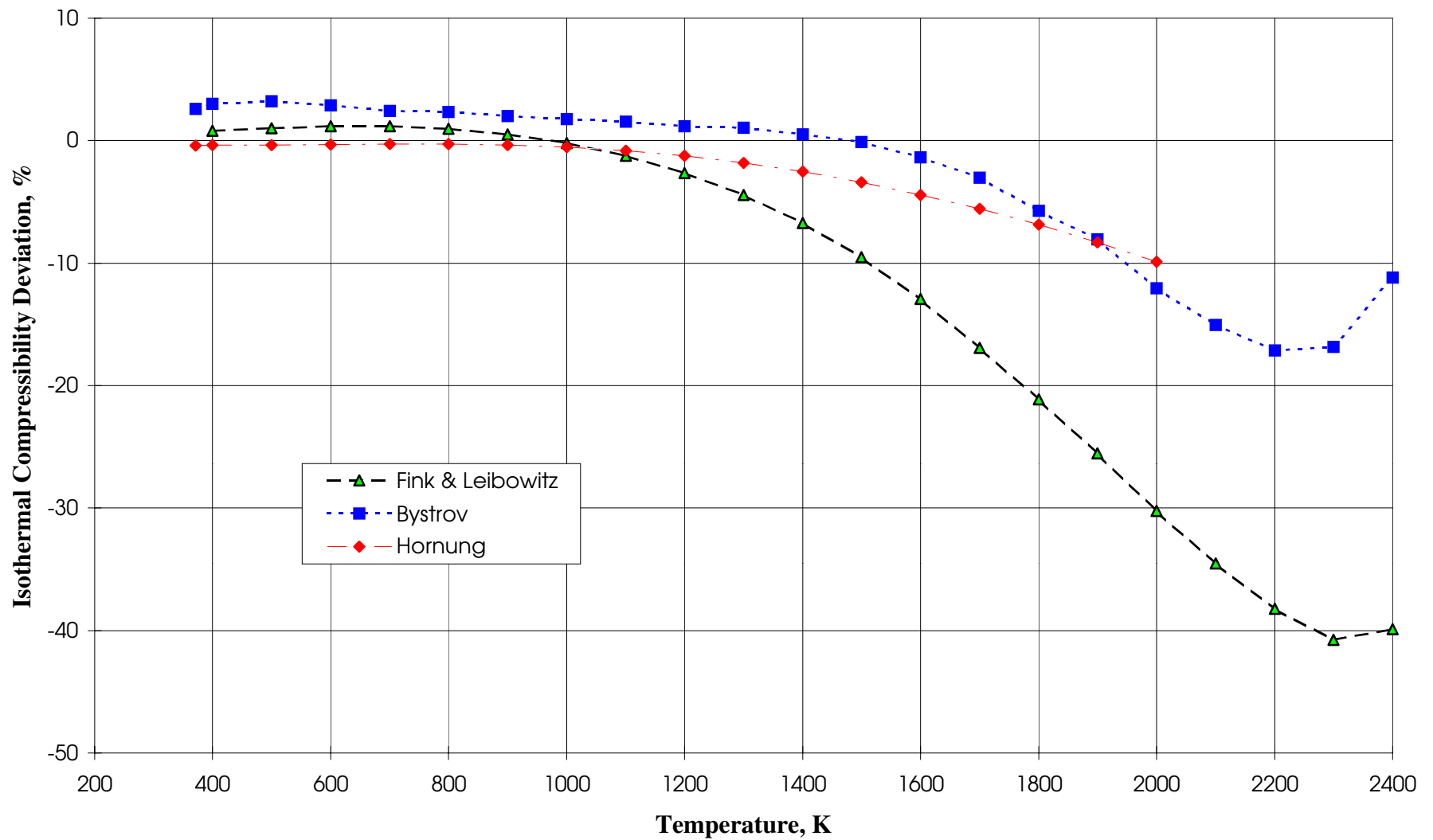
Fig. 1.4-13 Percent Deviations of the Recommended Values for the Isothermal Compressibility of Liquid Sodium from Values from Other Assessments
