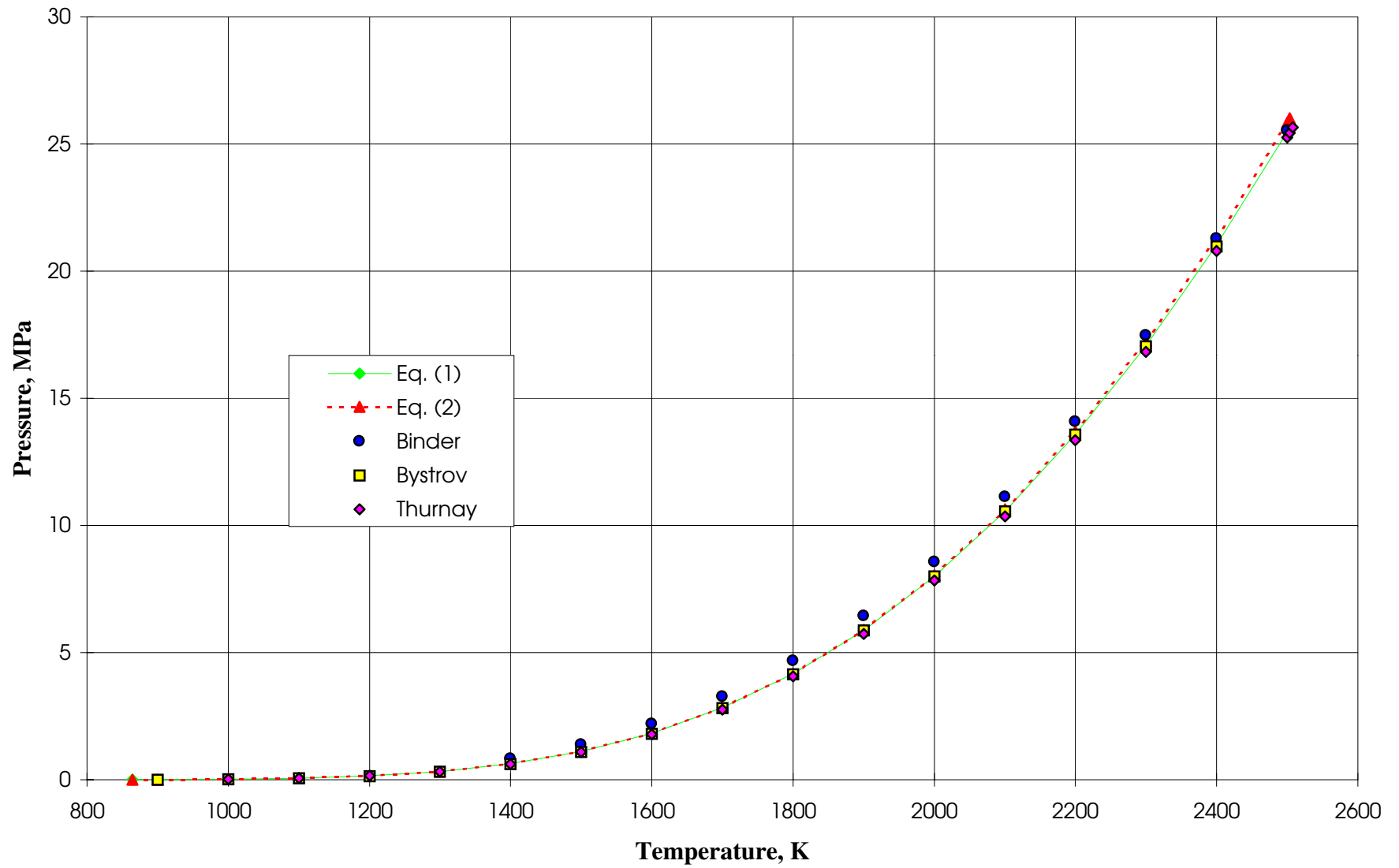
Fig. 1.2-4 Vapor Pressures Calculated from Various Recommended Equations
