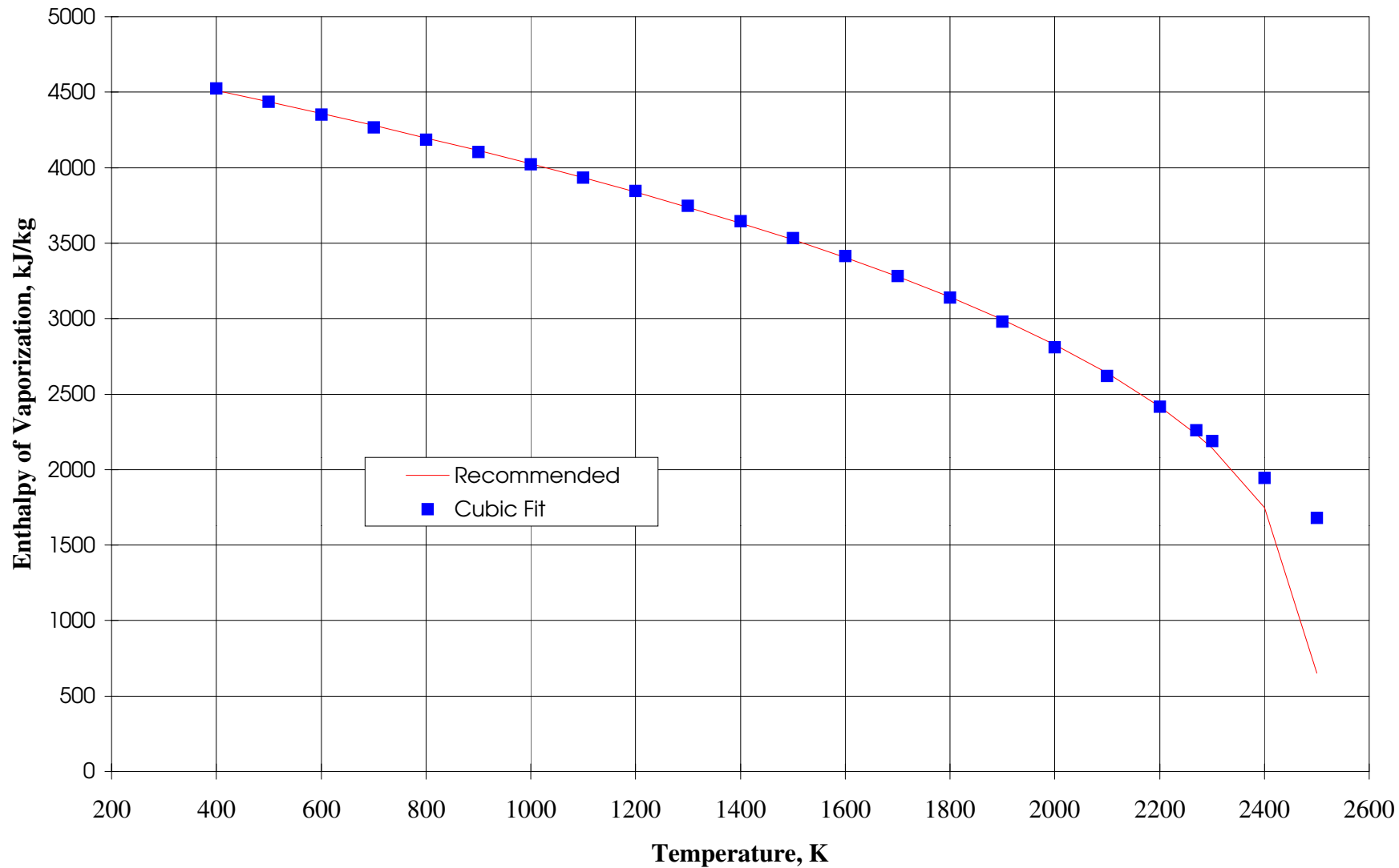
Fig. 1.2-11 Comparison of the Cubic Fit from the Recommended Values for the Enthalpy of Vaporization of Sodium
