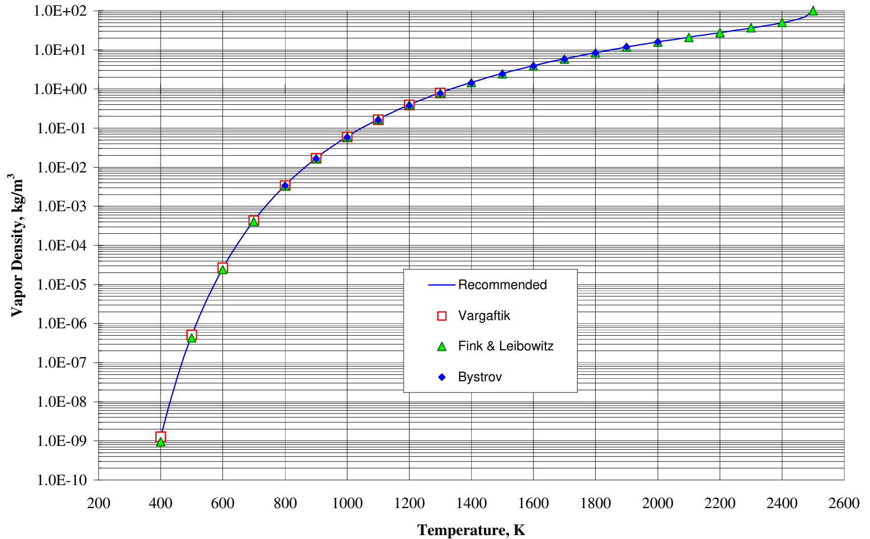
Fig 1.3-4 Comparison of Recommended Values for the Density of Sodium Vapor with Values from Other Assessments
