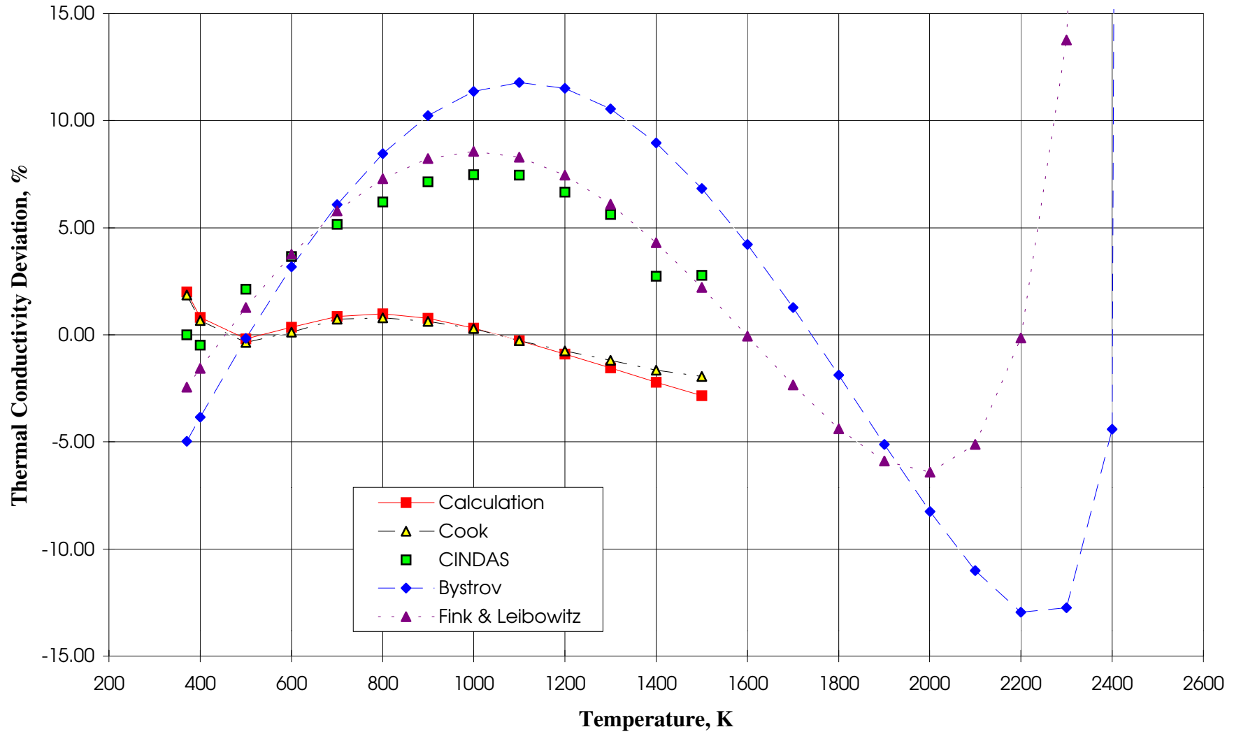
Fig. 2.1-13 Deviations of Values from Other assessments from Recommended Values of the Thermal Conductivity of Liquid Sodium
