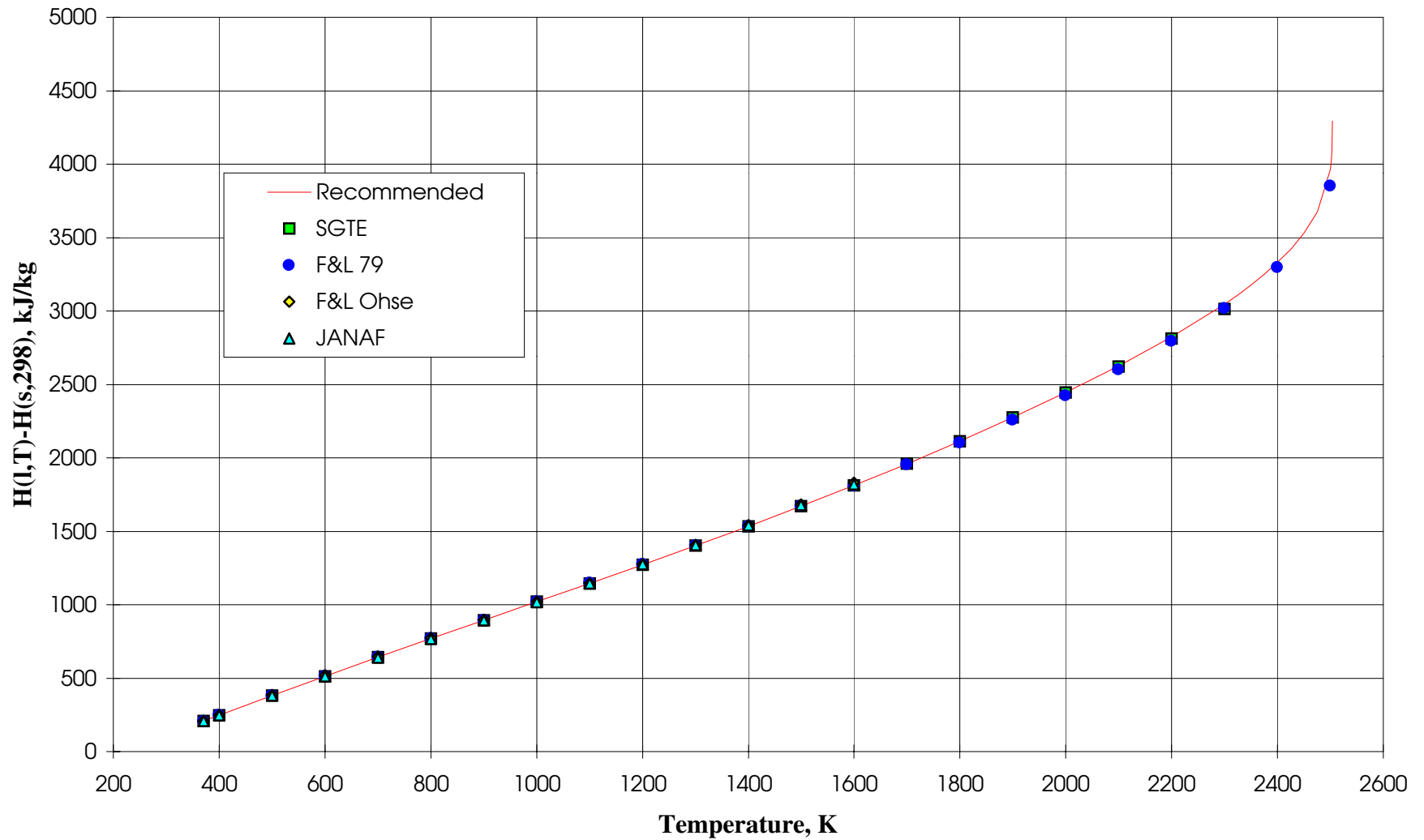
Fig. 1.1-2 Comparison of Recommended Values for the Enthalpy Increment of Liquid Sodium with Values from Other Assessments
