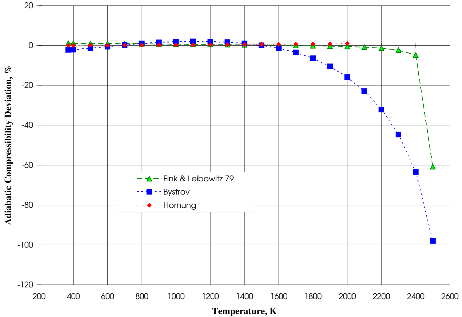
Fig. 1.4-4 Deviation of the Recommended Values for the Adiabatic Compressibility of Liquid Sodium from Values from Other Assessments
