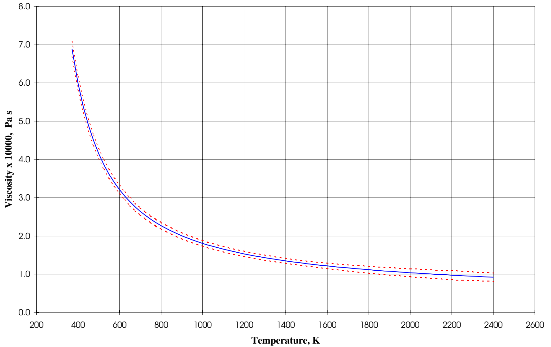
Fig. 2.2-1 Viscosity of Liquid Sodium
