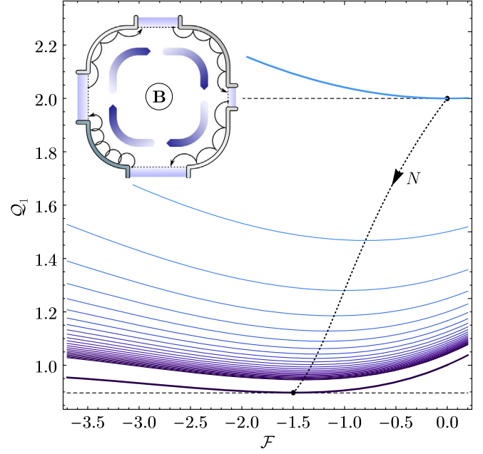
FIG. 2. Chiral transport. Bouncing orbits enforced by a strong magnetic field \mathbf{B} sustain clockwise-oriented currents between adjacent leads (inset). From top to bottom, the blue lines show the cost-precision ratio \mathcal{Q}_1 defined in (15) as a function of the rescaled bias increment \mathcal{F} for systems with N = 2, \dots, 25 terminals and for the limiting case N \rightarrow \infty . Interpolating between the minima of \mathcal{Q}_1 , the dotted line crosses the two dashed lines, respectively indicating the bounds (10) and (13), at N = 2 and N \rightarrow \infty .
