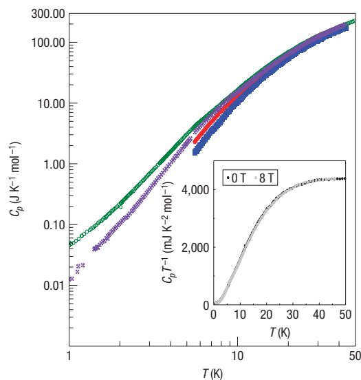
Figure 1 Temperature dependence of heat capacities of BEDT-TTF-based salts.
