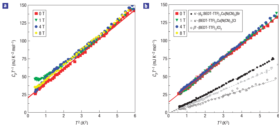
Figure 2 Low-temperature heat capacities of \kappa -(BEDT-TTF) 2 Cu 2 (CN) 3 . a, b , Data obtained for two samples under magnetic fields up to 8 T in C_p T^{-1} versus T^2 plots. b contains the data of the typical antiferromagnetic insulators \kappa -(BEDT-TTF) 2 Cu[N(CN) 2 ]Cl, deuterated \kappa -(BEDT-TTF) 2 Cu[N(CN) 2 ]Br and \beta' -(BEDT-TTF) 2 ICl 2 for comparison. The existence of a T -linear contribution even in the insulating state of \kappa -(BEDT-TTF) 2 Cu 2 (CN) 3 is clearly observed.
