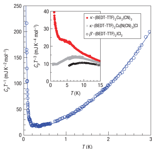
Figure 3 C_p T^{-1} versus T plot of the heat capacity for \kappa -(BEDT-TTF) 2 Cu 2 (CN) 3 . The solid curve shows the result of fitting to the formula C_p = A/T^2 + \gamma T + \beta T^3 . The obtained \gamma is 12 mJ K -2 mol -1 , which demonstrates the existence of continuous excitations from the ground state. The inset shows C_p T^{-3} versus T for \kappa -(BEDT-TTF) 2 Cu 2 (CN) 3 , \kappa -(BEDT-TTF) 2 Cu[N(CN) 2 ]Cl and \beta' -(BEDT-TTF) 2 Cl 2 .
