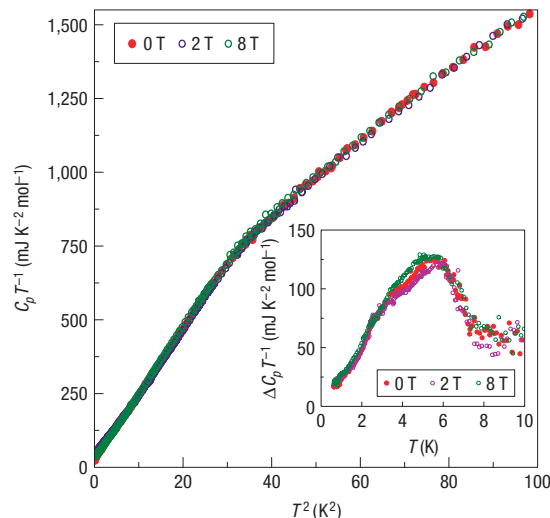
Figure 4 Temperature dependence of the heat capacity around the anomalous temperature of 6 K. C_p T^{-1} versus T^2 plots of the heat capacity of \kappa -(BEDT-TTF) 2 Cu 2 (CN) 3 under magnetic fields of 0 T (red), 2 T (purple) and 8 T (green). The inset shows the difference of the heat capacities of \kappa -(BEDT-TTF) 2 Cu 2 (CN) 3 and \kappa -(BEDT-TTF) 2 Cu(NCS) 2 , which highlights the hump structure around 6 K.
