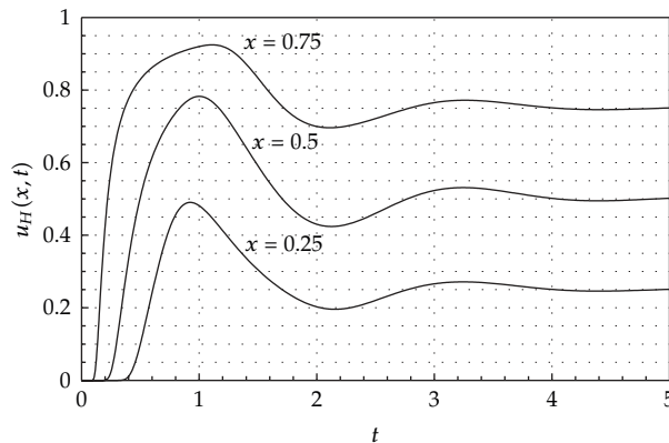
Figure 3: Displacements u_H(x, t) in a stress relaxation experiment as functions of time t at x \in \{0.25, 0.5, 0.75\} for t \in (0, 5) .
