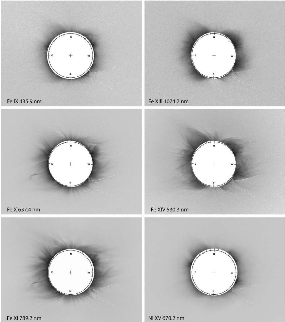
Fig. 7.— The same spectral line images as in Figure 6 processed with ACHF and shown as negatives. The Cone is also given by the dashed lines in all panels.
