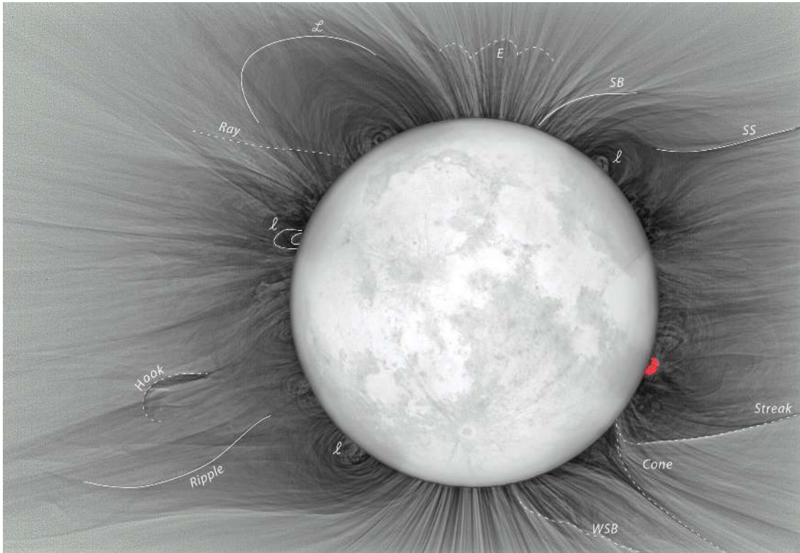
Fig. 3.— Same as Figure 2 with labels assigned to features, such as distinct rays, Ray , small scale loops, l , large-scale loops, L , the streamer stalk, SS , the streamer boundary, SB , the Hook , and the enhancement E . The Ripple , the wavy streamer boundary, WSB , the Streak and the Cone , are examples of structures resulting from prominence eruptions and the passage of CMEs through the corona prior to totality, as described later in Figure 9.
