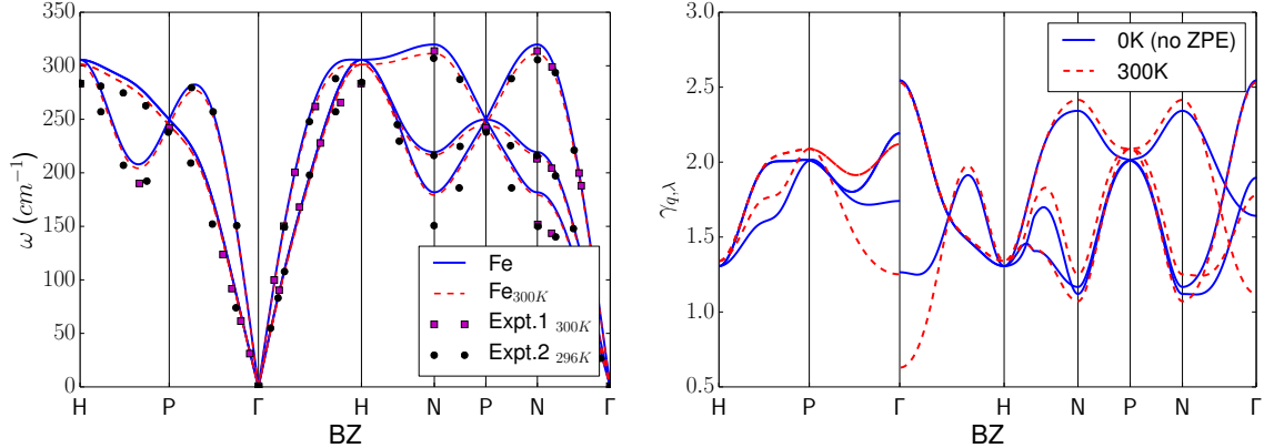
FIG. 5. (Left panel) Phonon dispersions along high-symmetry directions in the BZ calculated at the theoretical electronic equilibrium volume (blue solid line) and at the quasi-harmonic theoretical equilibrium volume at 300 K (red dashed line). The results (see also Fig. 1 in Supplemental Material a and Ref. 8 or Ref. 56 for comparison with previous theoretical data) are compared to experimental data at room temperature from Ref. 57 (Expt.1 – squares) and Ref. 58 (Expt.2 – circles). (Right panel) Grüneisen parameters calculated along the same path in the BZ and the same equilibrium volumes used for the phonon dispersion (blue solid line for the 0 K case and red dashed line for the 300 K case). The Grüneisen parameters are obtained computing the first derivative with respect to the volume of a cubic fit of the phonon frequencies.
