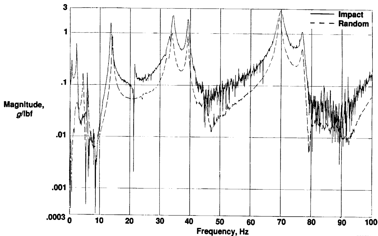
Figure 8. Comparison of frequency response plots for impact and random excitation at 400 °F.
