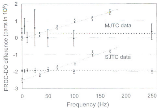
Fig. 3. FRDC measurement results. The upper pair of least-sum-squares (LSS) fit lines correspond to the MJTC. The lower pair of LSS fit lines are for the SJTC. Data from the Josephson source is shown with open squares, and data from the semiconductor source is shown with solid circles. The uncertainty shown is Type A, k = 2 .
