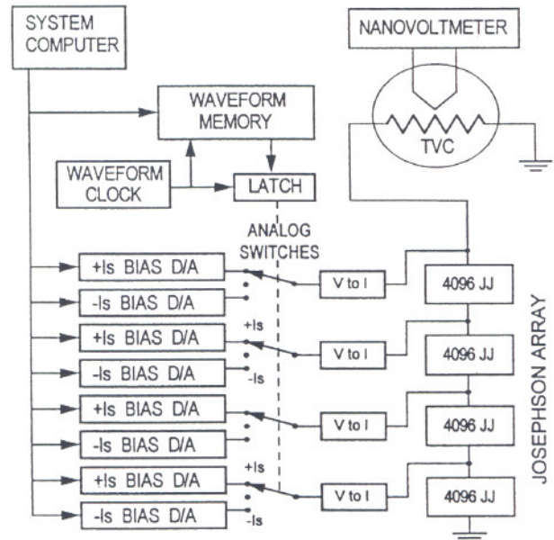
Fig. 2. Block diagram of the Josephson array system.
