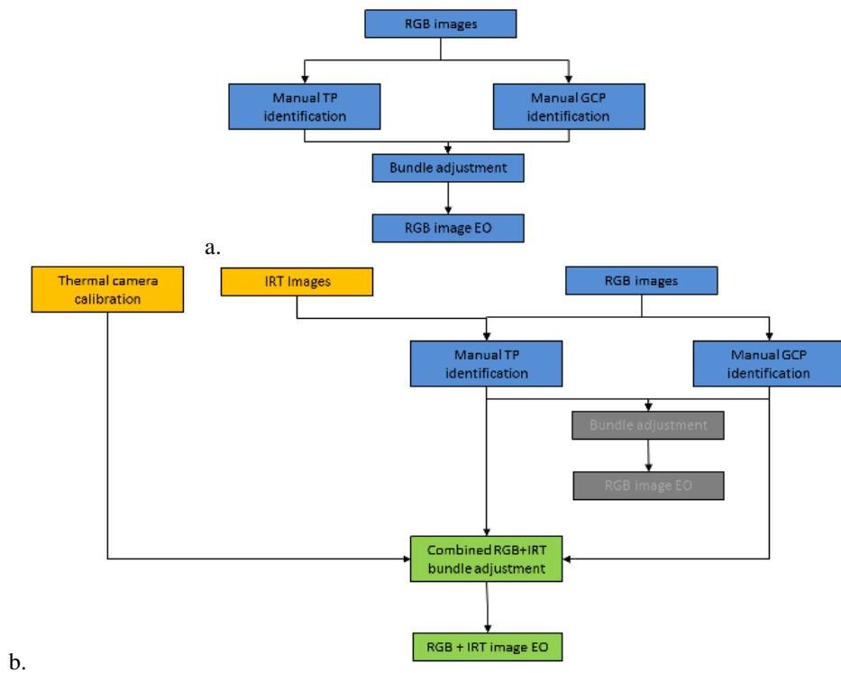
Figure 5 The first step of image orientation: only RGB images are processed (a); second step of image orientation: IRT images are added and a combined bundle adjustment is performed.
