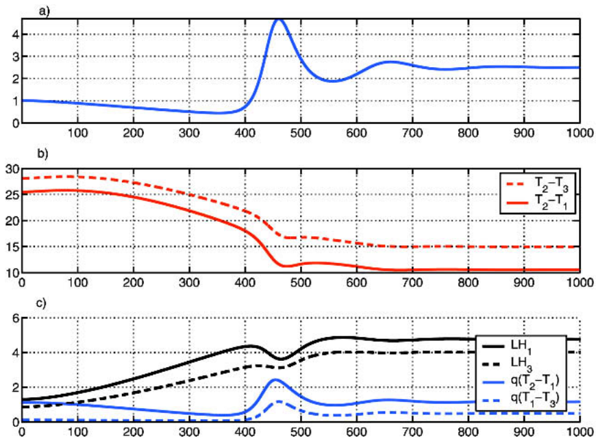
FIG. 2. (a) Evolution of the THC strength in units of q(0) for the subcritical case presented in Fig. 1. (b) Evolution of the meridional temperature gradient T_2 - T_1 and T_2 - T_3 in units of ^\circ\text{C} . (c) Evolution of the latent heat fluxes and the oceanic advection thermal forcings q(T_2 - T_1) (into box 1) and q(T_1 - T_3) (into box 3) in units of |\alpha q(0)[T_2(0) - 2T_1(0) + T_3(0)]| . Abscissas show elapsed time expressed in y.
