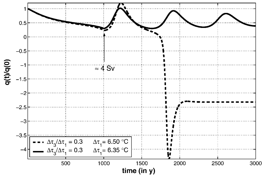
FIG. 7. Evolution of the THC strength under a super- and subcritical forcing to target temperatures.
