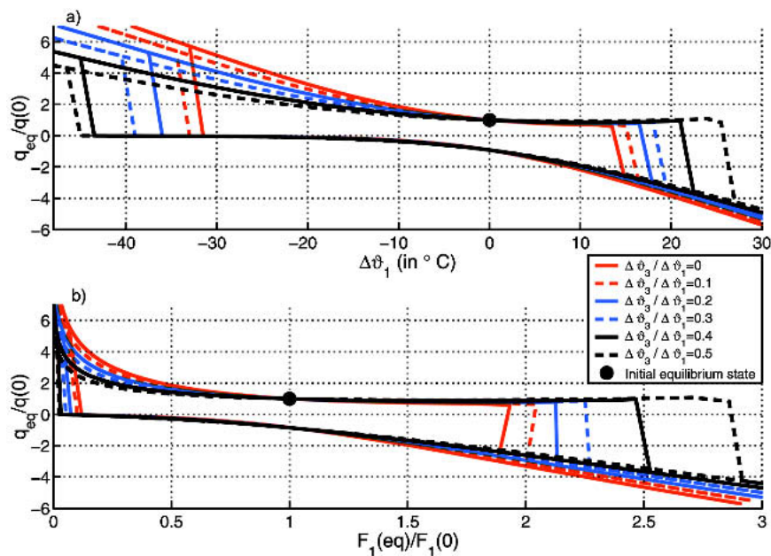
FIG. 5. Hysteresis graphs of the system with n = 1 for radiative temperature perturbations. (a) Radiative temperature change \Delta\vartheta_1 is considered as the relevant parameter. (b) Freshwater flux F_1 is considered as the relevant parameter.
