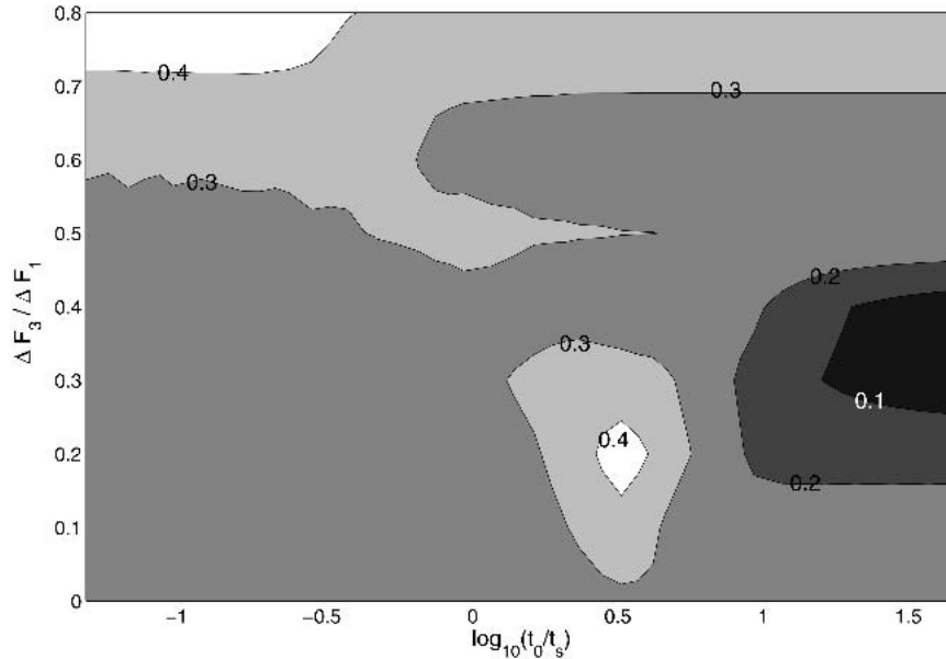
FIG. 6. Comparison between the stability of the mixed and flux BC uncoupled model to increases of the freshwater fluxes; contours of \Delta F_1^{\text{mix}}/\Delta F_1^{\text{flux}} .
