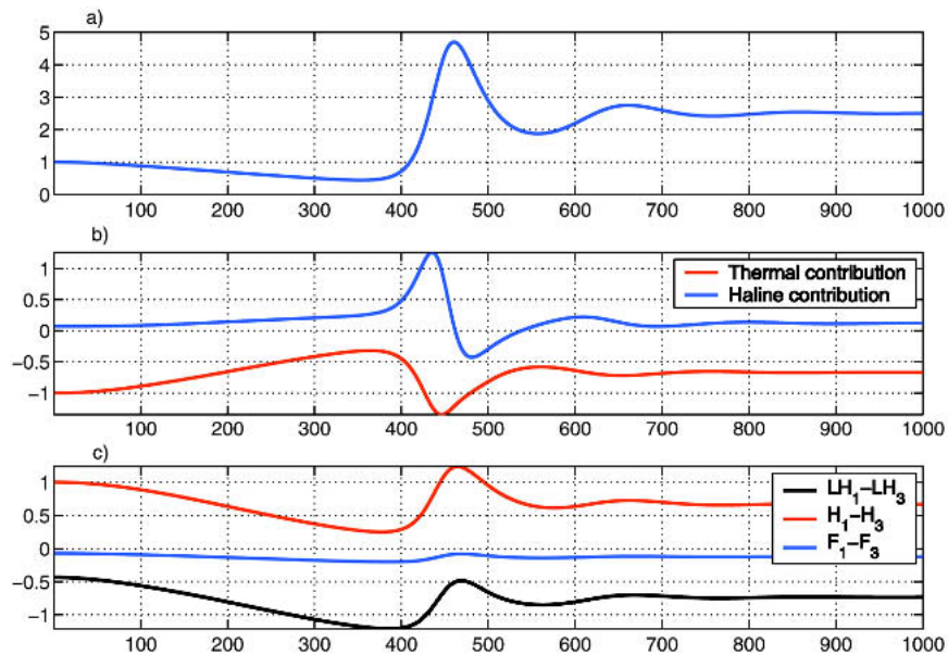
FIG. 3. (a) Evolution of the THC strength in units of q(0) for the subcritical case presented in Fig. 1. (b) Evolution of the thermal and haline oceanic advective forcings to the strength of the THC in units of |\alpha q(0) [T_2(0) - 2T_1(0) + T_3(0)] . (c) Evolution of the most relevant atmospheric contributions to the forcing to the strength of the THC [same units as in (b)]. Abscissas show elapsed time expressed in y.
