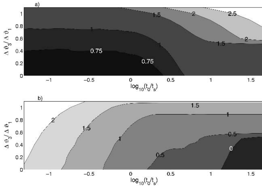
FIG. 6. Stability of the THC against perturbations to the radiative temperature with n = 1 . (a) Critical values of the total increase of the freshwater flux; contours of \log_{10}[\Delta\vartheta_1] , where \Delta\vartheta_1 is in ^{\circ}\text{C} . (b) Critical values of the rate of increase of the freshwater flux. Contours are of \log_{10}[\vartheta_1'] , where \vartheta_1' is in ^{\circ}\text{C } t_s^{-1} and t_s is the advective time.
