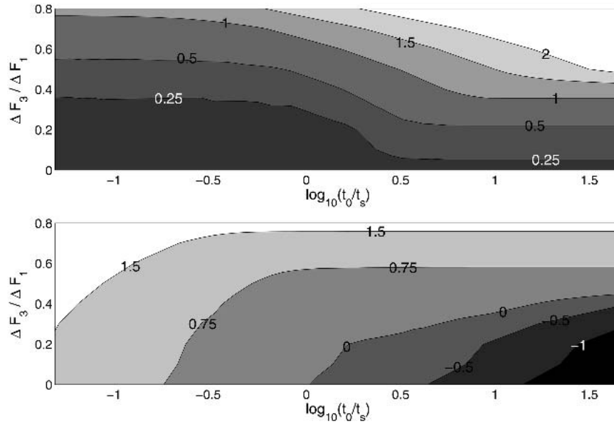
FIG. 4. Stability of the THC against freshwater flux perturbations. (a) Critical values of the total increase of the freshwater flux; contours of \log_{10}[\Delta F_1/F_1(0)] . (b) Critical values of the rate of increase of the freshwater flux; contours of \log_{10}[F_1't_0/F_1(0)] , where t_0 is the total length of forcing.
