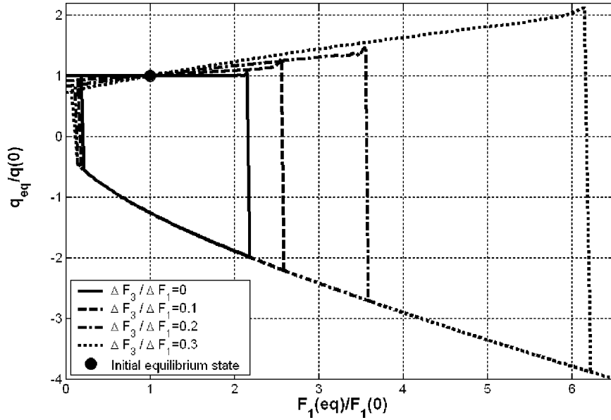
FIG. 3. Hysteresis graph of freshwater flux forcings.
