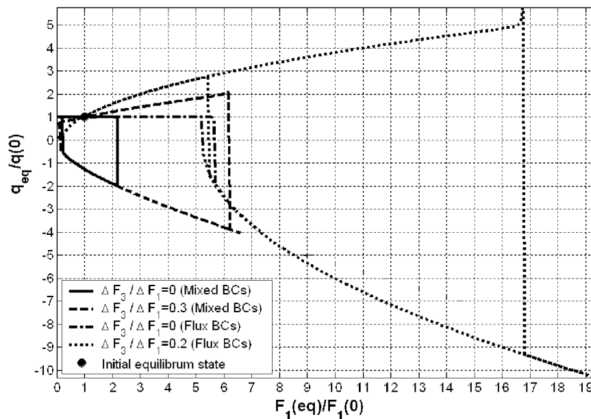
FIG. 5. Comparison between the stability of the mixed and flux BC uncoupled model to increases of the freshwater fluxes; hysteresis graphs.
