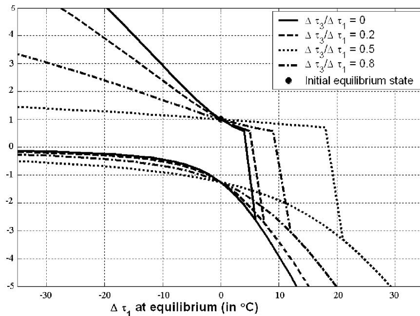
FIG. 8. Hysteresis graph of the target temperature forcings.
