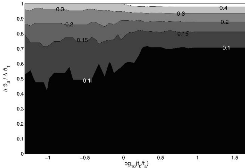
FIG. 9. Sensitivity to the low-to-high-latitude radiative forcing ratio TRRF of the critical values of the total increase of the radiative temperatures; contours are of \log_{10}[Z_C(\text{TRRF} = 1.0) / Z_C(\text{TRRF} = 2.0)] .
