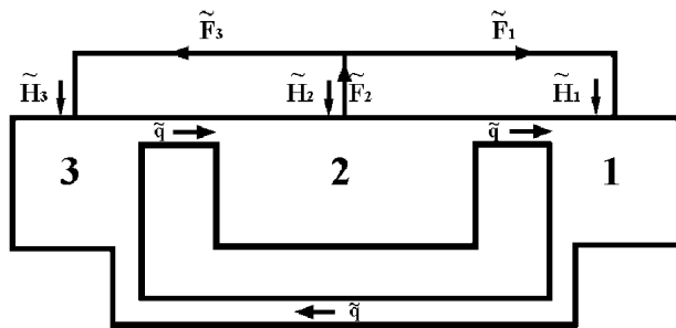
FIG. 1. Schematic picture of the interhemispheric box model.
