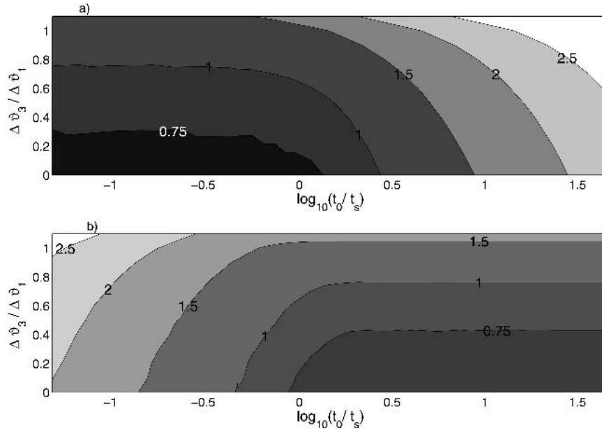
FIG. 7. Stability of the THC against perturbations to the radiative temperature with n = 3 . (a) Critical values of the total increase of the freshwater flux; contours are of \log_{10}[\Delta \vartheta_1] , where \Delta \vartheta_1 is in ^{\circ}\text{C} . (b) Critical values of the rate of increase of the freshwater flux; contours are of \log_{10}[\vartheta_1'] , where \vartheta_1' is in ^{\circ}\text{C } t_s^{-1} and t_s is the advective time.
