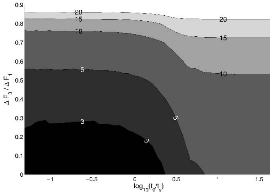
FIG. 9. Stability of the THC against target temperature perturbations. Critical values of the total increase of the target temperature \tau_1 ; contours of \Delta\tau_1 in ^{\circ}\text{C} .
