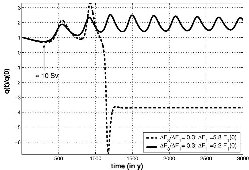
FIG. 2. Evolution of the THC strength under a super- and subcritical freshwater flux forcing.
