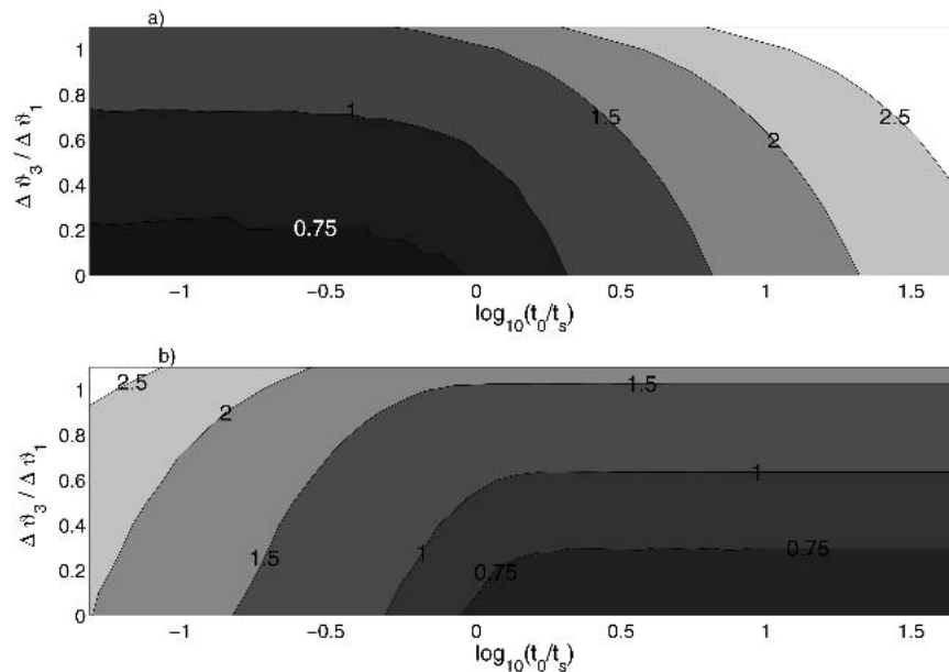
FIG. 8. Stability of the THC against perturbations to the radiative temperature with n = 5 . (a) Critical values of the total increase of the freshwater flux; contours are of \log_{10}[\Delta \vartheta_1] , where \Delta \vartheta_1 is in ^{\circ}\text{C} . (b) Critical values of the rate of increase of the freshwater flux; contours are of \log_{10}[\vartheta_1'] , where \vartheta_1' is in ^{\circ}\text{C } t_s^{-1} and t_s is the advective time.
