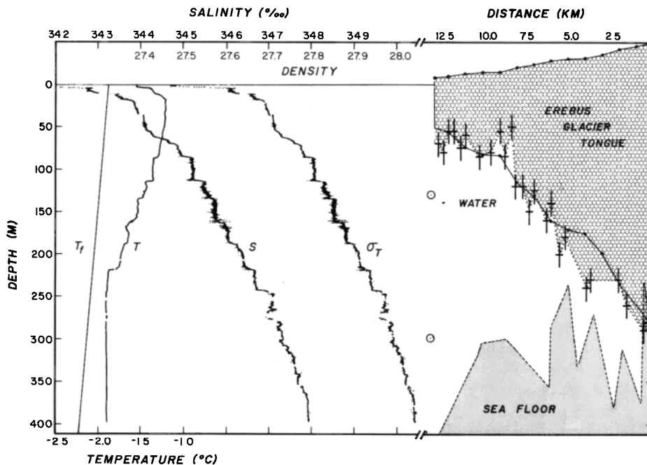
Fig. 3. (Left) Temperature T , salinity S , and density \sigma , profiles from Glacier station 217, located a few hundred meters south of the western terminus of Erebus Glacier Tongue (EGT). The in situ freezing point ( T_f ) is after Fujino et al. [1974]. (Upper right) A vertical section along the EGT center line. The upper surface of the floating glacier is defined at 1 km intervals ( \pm 100 m) to \pm 2 m in the vertical. The equilibrium basal profile (dash-dot line) is calculated for free flotation of a slab of mean density 0.87 \text{ Mg m}^{-3} . The January 1978 radar basal profile (dotted line) has a vertical resolution of \pm 15 m as shown by the error bars. North and south edges of the EGT are approximately 40% thinner than the center line profile. (Lower right) Dashed line connects line soundings of the sea floor north and south of the EGT. Circled dots are bottom depths on CTD stations 218, and 219. The EGT moves off Ross Island into water that is 225–275 m deep. The irregular sea floor beneath the EGT continues for at least another 5 km west of its terminus (DMA chart 29322, Cape Royds to Hut Point).
