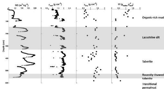
Figure 4. Depth profiles for magnetic susceptibility (MS), wet bulk density ( \rho_{\text{wet}} ), dry bulk density ( \rho_{\text{dry}} ), and gravimetric water content ( W ) in the Vault Lake sediment core. Two MS values at 95.4 and 405.4 cm were -493.1 and -488.0 \text{ m}^3 \text{ kg}^{-1} , respectively (not shown).
