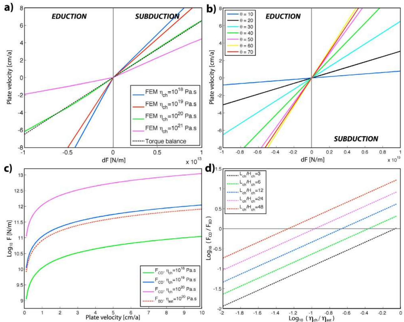
Figure 9. (a) Plate velocity for variable force difference ( dF ) (using \eta_{ast} = 10^{20} Pa.s and \theta = 30^\circ ). The solid lines represent the solution obtained from the 2D simulations for different subduction channel viscosities ( \eta_{ch} ). The dotted line is the prediction of the torque balance approach for an isoviscous mantle. (b) Sensitivity of plate velocity to the slab dip angle for variable force difference values. This was computed using the torque balance model. (c) Magnitude of the basal drag (red) and channel drag forces (blue) estimated for our 2D setup as a function of plate velocity. These estimations assume a Couette flow in the asthenosphere and the subduction channel. (d) Efficiency of the subduction channel drag over the basal drag for various channel aspect ratios and channel/asthenosphere viscosity contrast.
